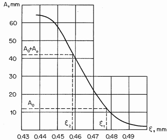
Figure 50 Signal amplitude as a function of the knife-edge position.
