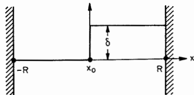
Figure 149 Wave front with a discontinuity at point x_0 .
