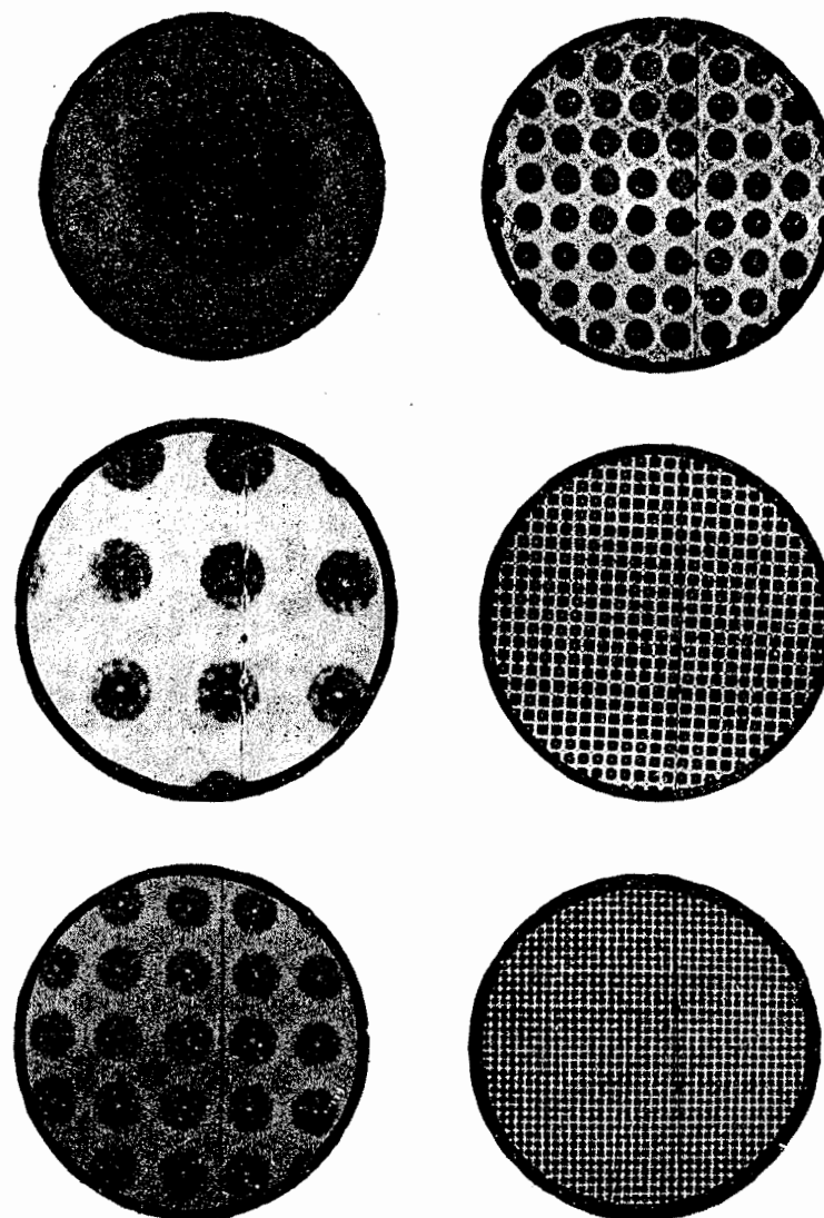
Figure 68 Schlieren patterns for various defocusing of the point grid.
