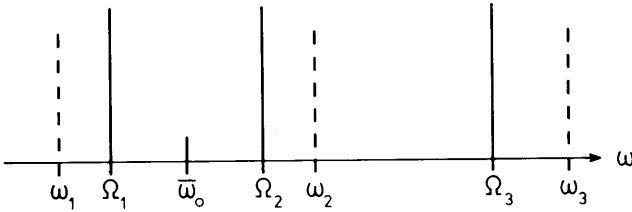
Fig. 6.2. Frequency locking. Scheme of mode frequencies. The abscissa represents the circular frequency. \omega_0 is the atomic center frequency. \omega_1, \omega_2, \omega_3 are the mode frequencies in the empty resonator; \Omega_1, \Omega_2, \Omega_3 are the actual mode frequencies when laser action takes place but still without the coupling which causes frequency locking.
