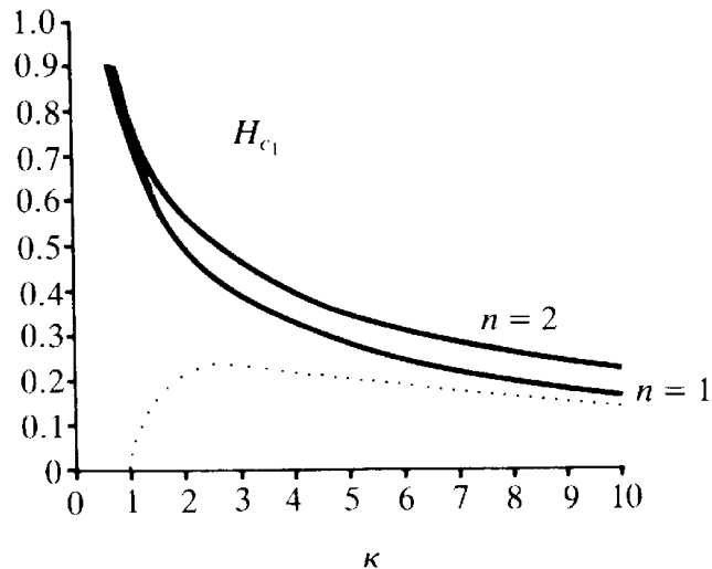
FIG. 3.4. The critical field H_{c_1} at which a vortex line of strength n forms when it first invades a type II superconductor as a function of the parameter \kappa . The dotted line indicates the asymptotic result (1/2\kappa) \log \kappa of Eq. (3.89). The magnetic field H_{c_1} is measured in units of \sqrt{2}H_c where H_c is the magnetic field at which the magnetic energy equals the condensation energy.
