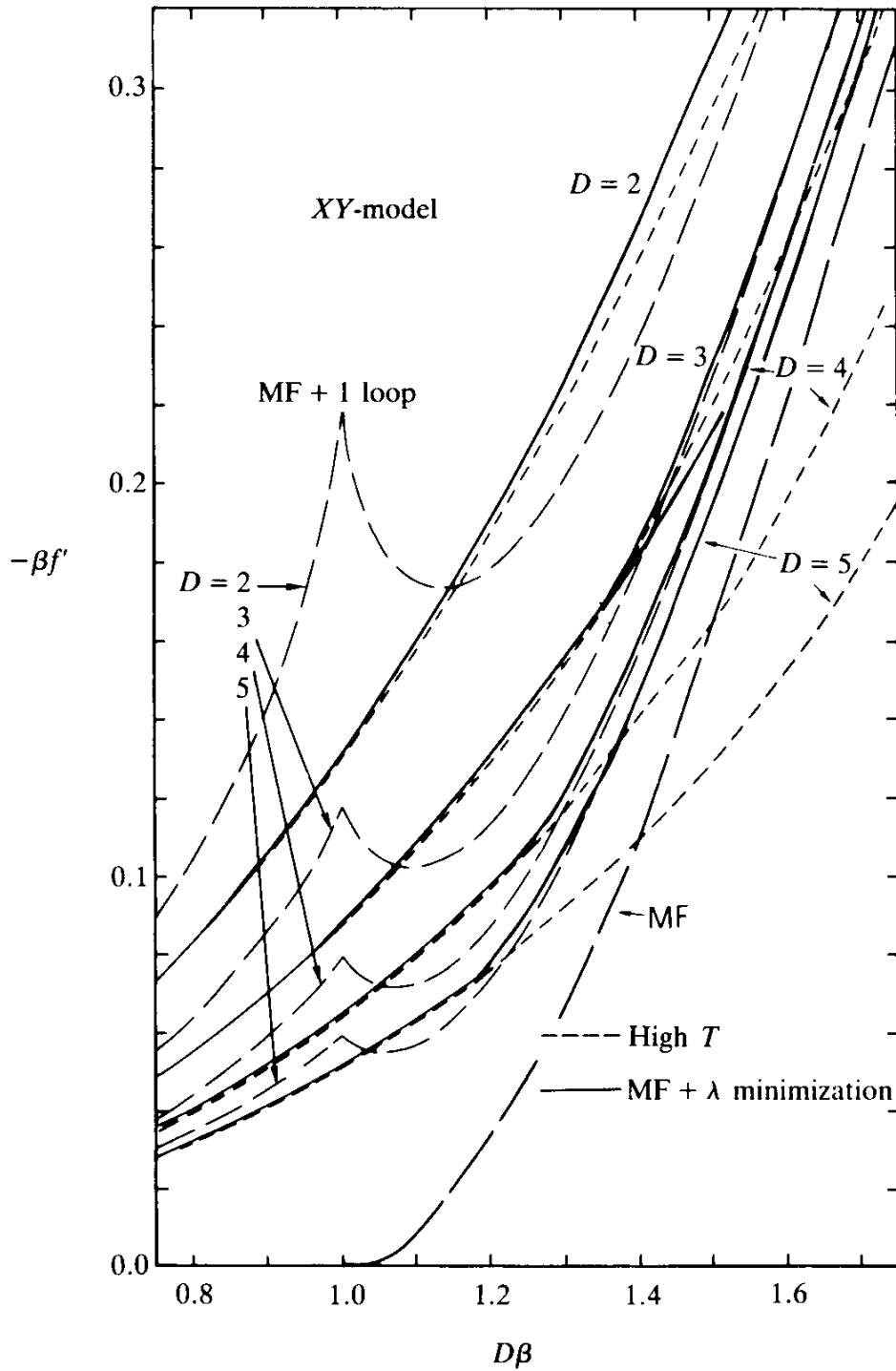
FIG. 4.5. The same curves as in Fig. 4.4 plotted for various dimensions. We see that for D \rightarrow \infty the mean field curves become exact. In addition, there are solid curves ( \lambda minimization) which will be discussed later on in Section 5.7.
