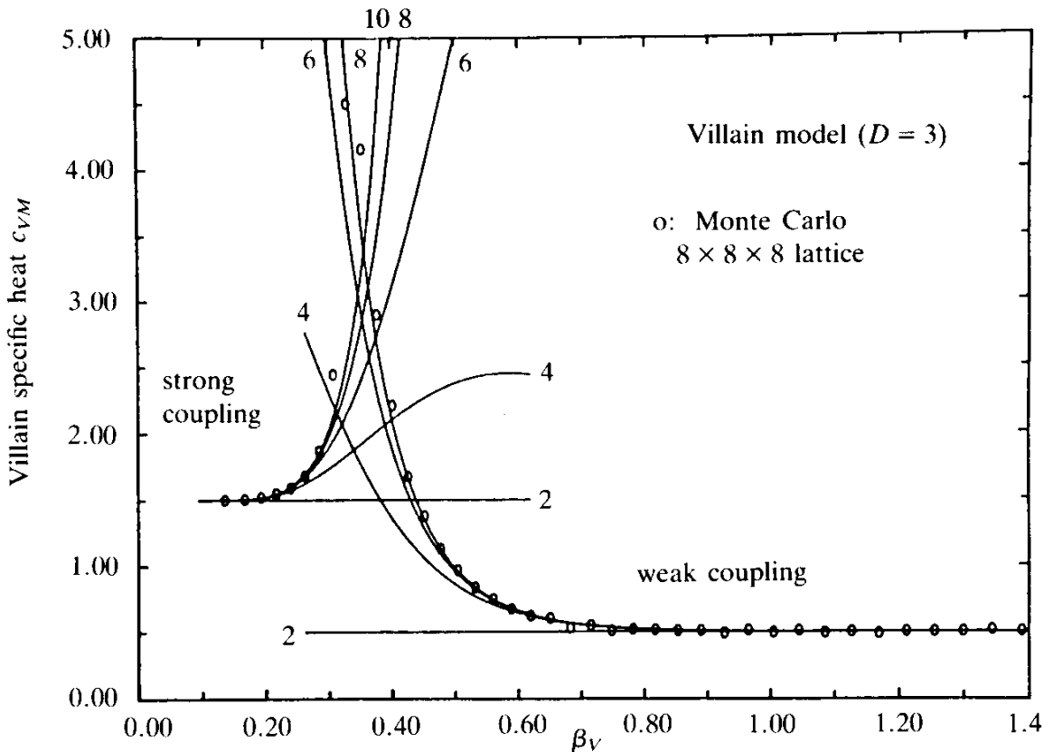
FIG. 7.7. Specific heat of the D=3 Villain model as compared with high- T , low- T expansions and Monte Carlo data (same as in Fig. 7.6). We see clearly the transition at \beta_{Vc} \approx 0.33 .
