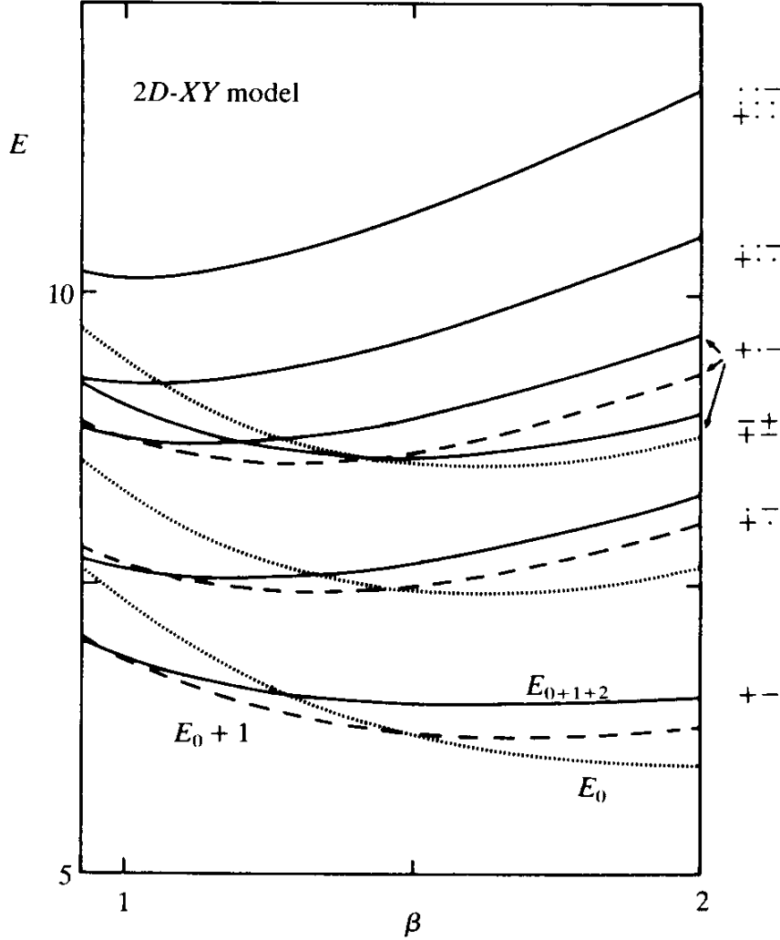
FIG. 11.11. Loop expansion of bound vortex energies (zero loop E_0 , up to 1-loop E_{0+1} , and up to 2-loop E_{0+1+2} ) as a function of inverse temperature \beta .
