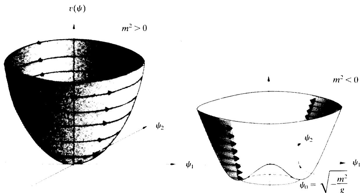
FIG. 1.5. The effective potential of the superfluid as a function of the order parameter \psi = \psi_1 + i\psi_2 for T > T_c ( m^2 > 0 ) and T < T_c ( m^2 < 0 ). The arrows indicate the invariance under phase rotations \psi \rightarrow e^{i\alpha} \psi .
