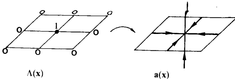
FIG. 6.2. Illustration of the pure gauge term a_i(\mathbf{x}) = \nabla_i \Lambda(\mathbf{x}) with \Lambda = \text{integer} which adds to the vector potential a pure "sink" (since \bar{\nabla} \times \mathbf{a}(\mathbf{x}) = 0 ).
