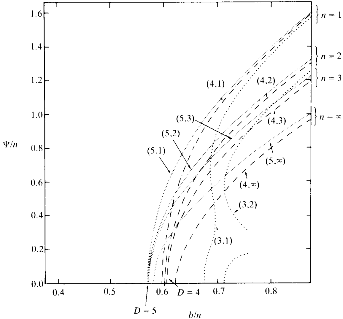
FIG. 5.10. The order parameter \Psi/n = (2b/n) \langle u \rangle in the O(n) spin model for various dimensions and values of n from the two-loop effective energy (up to second order in 1/D ). For low D and large N the (unphysical) first order, transition shows up in a concave or a missing piece in the solution.
