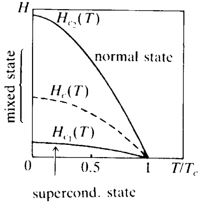
FIG. 3.6. The temperature behavior of the critical magnetic fields of a type II superconductor: H_{c1} (when the first vortex line invades), H_{c2} (when superconductivity is destroyed in comparison with the field) and H_c (when the magnetic field energy is equal to the condensation energy).
