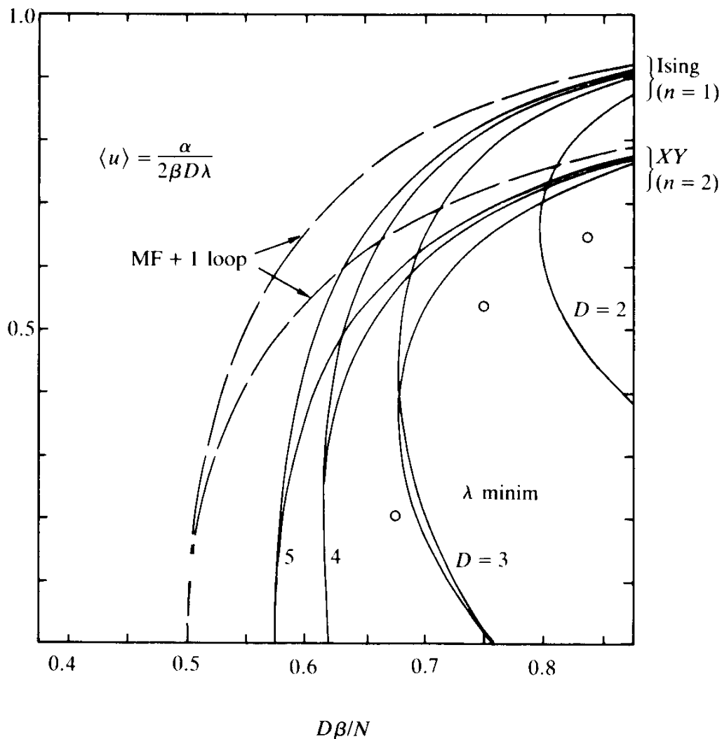
FIG. 5.7. The order parameter \langle e^{i\gamma} \rangle = \langle U \rangle of the XY model in the critical regime, in the mean-field-plus-one-loop approximation (which plotted against D\beta is independent of D ) and after minimizing in the additional parameter \lambda explained in Section 5.7. The circles are Monte Carlo data on a 16 \times 16 \times 16 lattice. We see that the \lambda method removes part of the discrepancy. The D = 3 curve still has an unphysical first order “belly.” For comparison, we also have drawn the theoretical curves of the Ising model.
