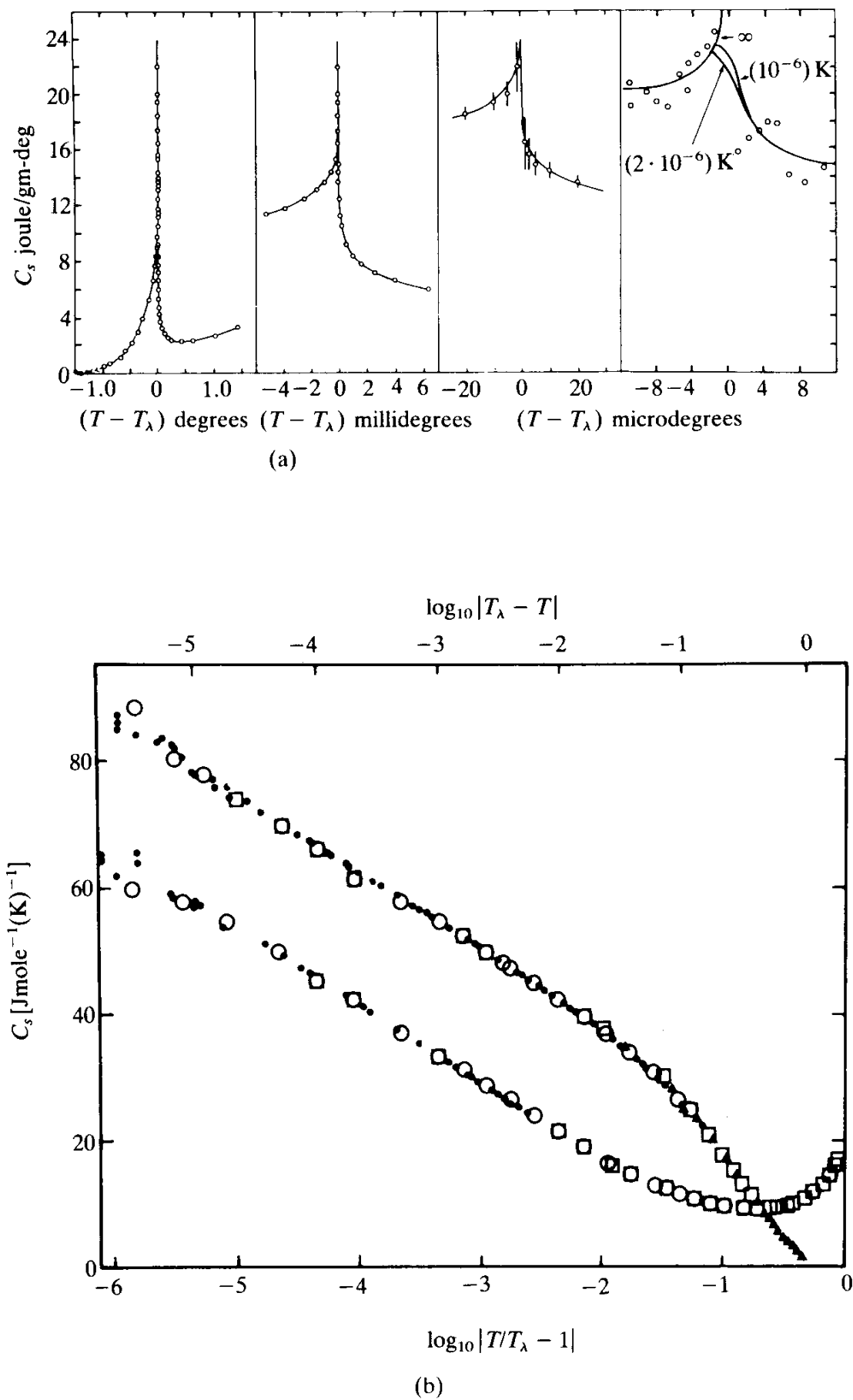
FIG. 4.11. The experimental specific heat of Fairbank et. al (a) and Ahlers (b) (see Notes and References).
