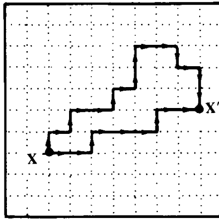
FIG. 9.1. Two possible strings of "magnetic flux" connecting a monopole at \mathbf{X} with an antimonopole at \mathbf{X}' and satisfying (9.5). For simplicity we plot only a planar configuration.
