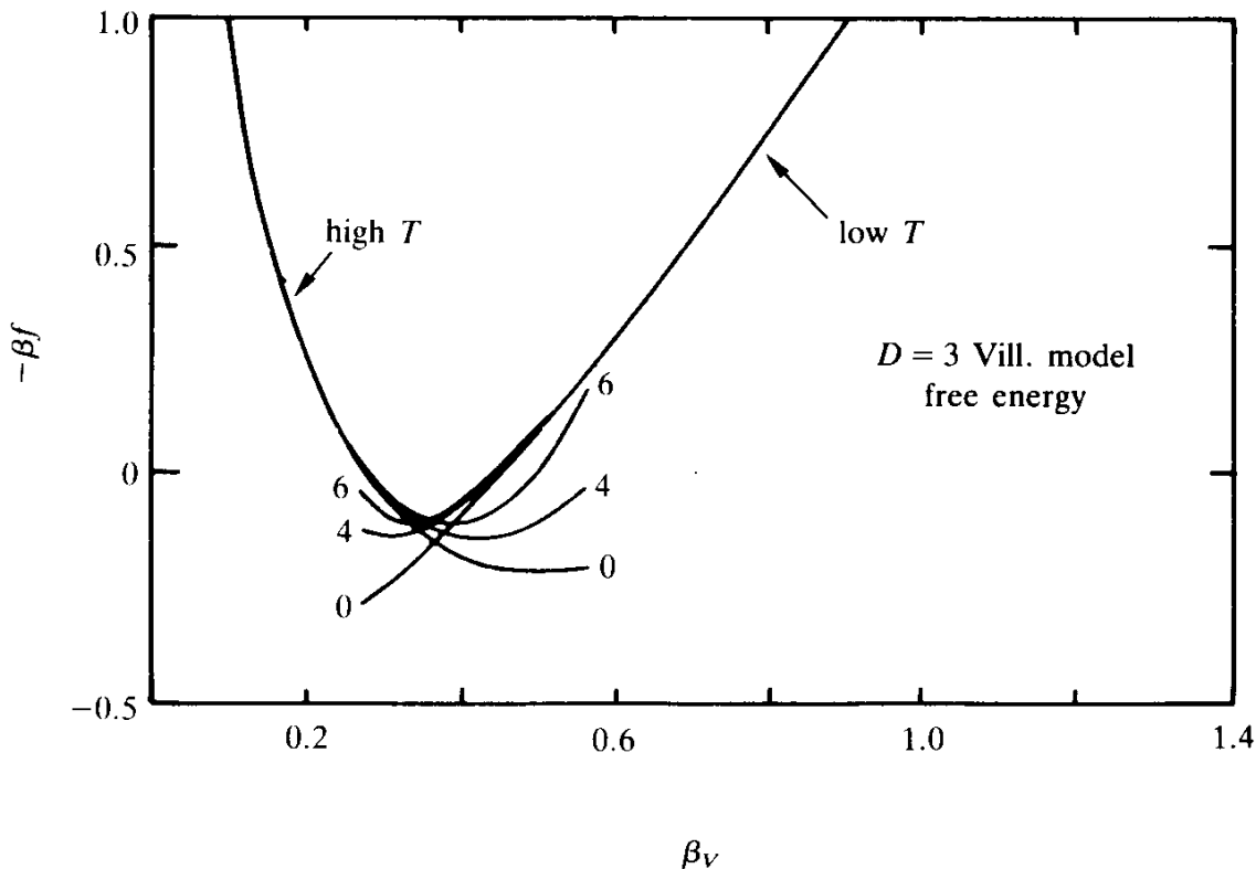
FIG. 7.5. Free energy of the D = 3 Villain model in the high and low temperature expansions. The curves show the contribution of the different low order loop diagrams (superflow loops for high- and vortex loops for low temperatures). The intersection of the two expansions gives a critical point \beta_c \approx 0.35 (compare with the Monte Carlo value of 0.333).
