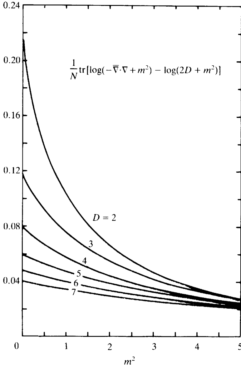
FIG. 6.4. The fluctuation determinant \int (d^D k / (2\pi)^D) \log(\vec{K} \cdot \vec{K} + m^2) on a simple cubic lattice as a function of m (with \log(2D + m^2) subtracted).
