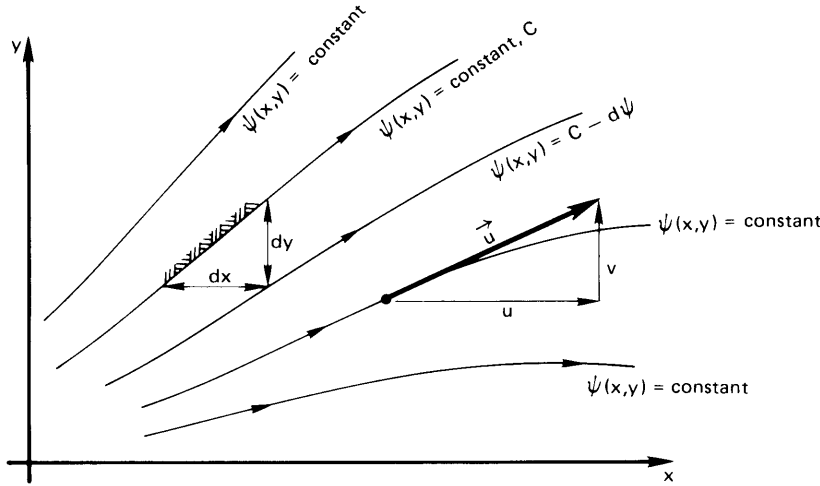
Figure 6.7 A steady, incompressible, two-dimensional flow field represented by streamlines, or lines of constant \psi .
