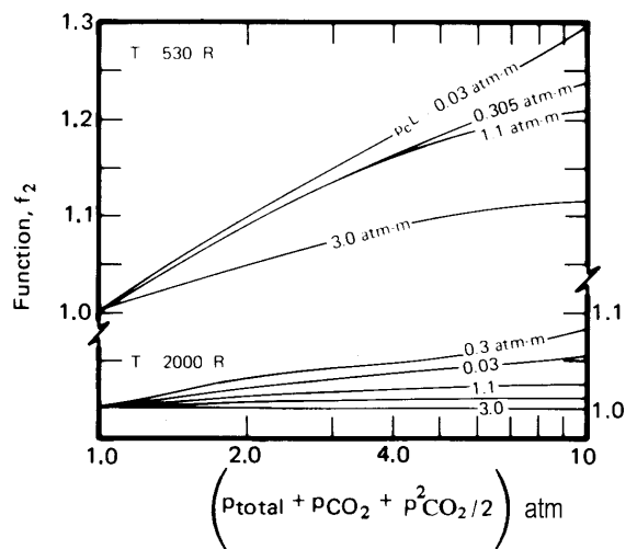
Figure 10.23 Functions used to predict \varepsilon_g = f_1 f_2 for \text{CO}_2 in air. All pressures in atmospheres.
