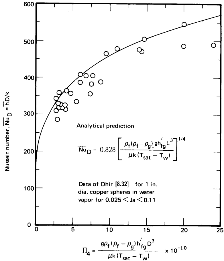
Figure 8.10 Correlation of the data of Dhira [8.32] for laminar film condensation on spheres at one value of Pr and for a range of \Pi_4 and Ja , with properties evaluated at (T_{sat} + T_w)/2 . Analytical prediction from [8.33].
