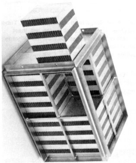
c) The basic 1 ft. \times 1 ft. \times 2 ft. module for a waste heat recuperator. It is a plate-fin, gas-to-air cross-flow heat exchanger with neither flow mixed.
