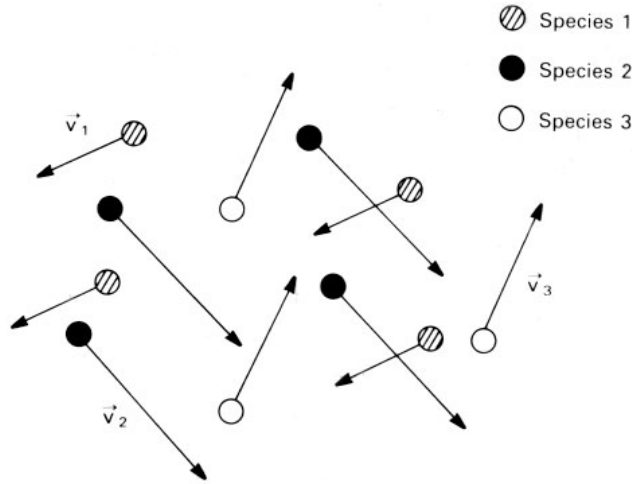
Figure 11.3 Molecules of different species in a mixture moving with different average velocities. The velocity \bar{v}_i is the average over all molecules of species i .
