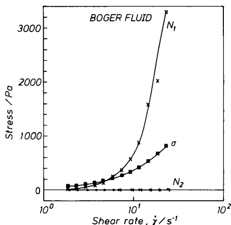
Fig. 4.5 Viscometric data for a Boger fluid: 0.184% polyisobutylene in a mixture of kerosene and polybutene (B.P. Hyvis 30). 25 °C.
