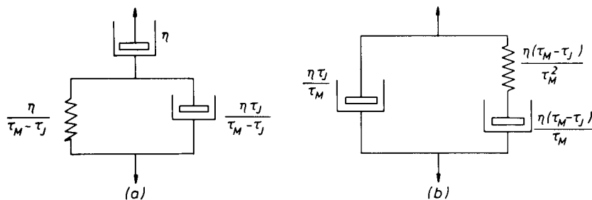
Fig. 3.5 Spring-dashpot equivalents of the Jeffreys model. The values of the constants of the elements are given in terms of the three material parameters of the model (eqn. 3.15).
