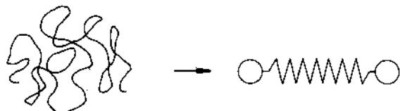
Fig. 6.8 The dumbbell approximation. The elastic behaviour is represented by a spring and the sites of the frictional drag are located at the ends of the spring.
