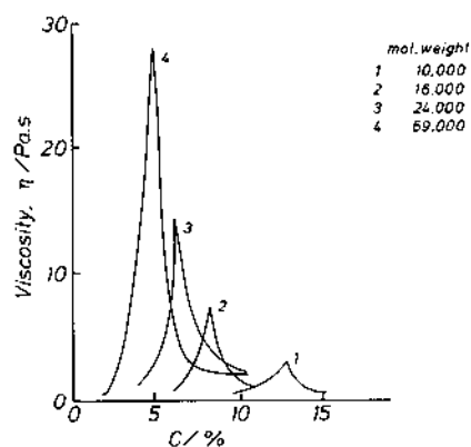
Fig. 6.6 Dependence of viscosity on concentration for solutions of poly(p-benzamide) in dimethyl acetamide at 20°C. The liquid-crystalline state occurs to the right of the maxima in the curves (from Vinogradov and Malkin 1980, p. 196).
