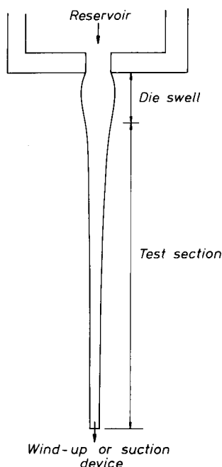
Fig. 5.7 Schematic diagram of the spin-line rheometer.
