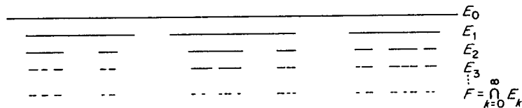
Figure 4.1 An example of the general construction of a subset of \mathbb{R}
