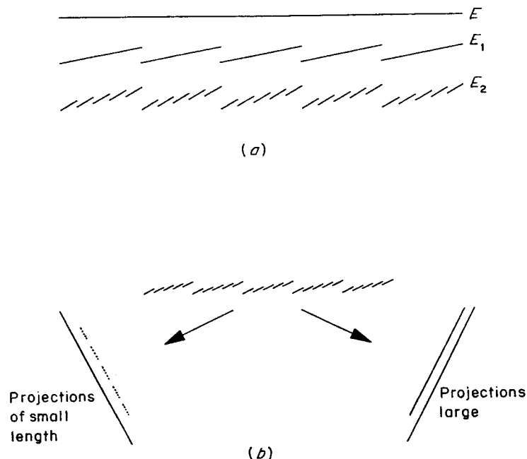
Figure 6.3 (a) The 'iterated Venetian blind' construction. (b) Projections in certain bands of directions have large lengths, whilst projections in other bands of directions have very small lengths
