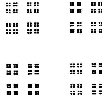
Figure 7.2 The product F \times F , where F is the middle third Cantor set. In this case, \dim_{\text{H}} F \times F = 2 \dim_{\text{H}} F = 2 \log 2 / \log 3
