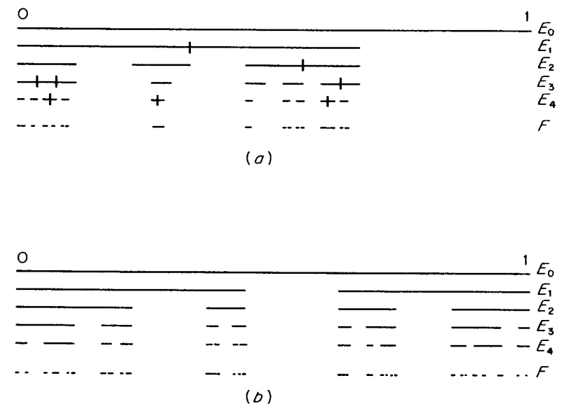
Figure 15.2 Two random versions of the Cantor set. In (a) each interval is divided into three equal parts from which some are selected at random. In (b) each interval is replaced by two subintervals of random lengths
