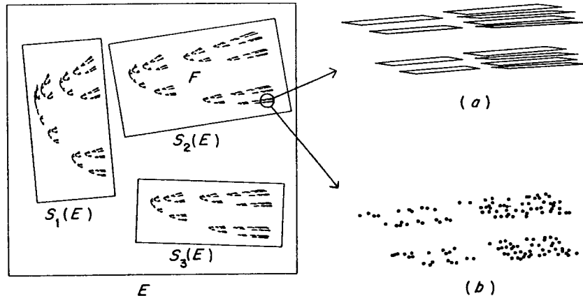
Figure 9.3 Two ways of computer drawing the fractal F , invariant under the three affine transformations S_1 , S_2 and S_3 which map the square onto the rectangles. In method (a) the 3^k parallelograms S_k(S_{i_1}(\dots(S_{i_k}(E)))) for i_j = 1, 2, 3 are drawn ( k=6 here). In method (b), the sequence of points x_k is plotted by choosing S_{i_k} at random from S_1 , S_2 and S_3 for successive k and letting x_k = S_{i_k}(x_{k-1})
