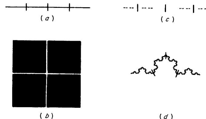
Figure 0.9 Division of certain sets into four parts. The parts are similar to the whole with ratios: \frac{1}{4} for line segment (a); \frac{1}{2} for square (b); \frac{1}{9} for middle third Cantor set (c); \frac{1}{3} for von Koch curve (d)
