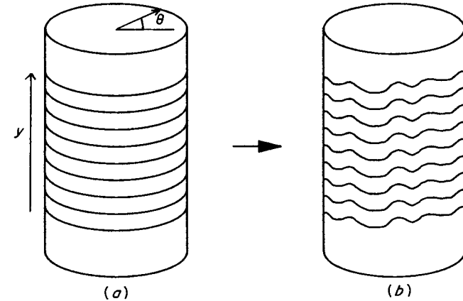
Figure 13.16 (a) Invariant circles for the mapping f(\theta, y) = (\theta + 2\pi\omega \pmod{2\pi}, y) . (b) If \omega is not 'too rational', a small perturbation of the mapping to f(\theta, y) = (\theta + 2\pi\omega \pmod{2\pi}, y + g(\theta)) distorts the circles to a family of smooth invariant curves
