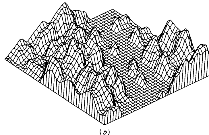
Figure 16.3 Index- \alpha fractional Brownian surfaces: (a) \alpha = 0.95 , dimension = 2.05; (b) \alpha = 0.8 , dimension = 2.20
