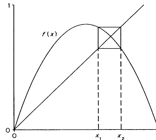
Figure 13.2 The logistic map f(x) = \lambda x(1 - x) for \lambda = 3.38 . Note the period-2 orbit x_1, x_2 with f(x_1) = x_2 and f(x_2) = x_1 .
