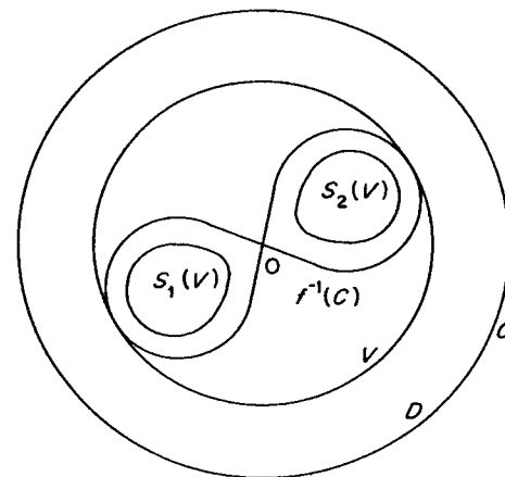
Figure 14.4 Proof of Theorem 14.15
