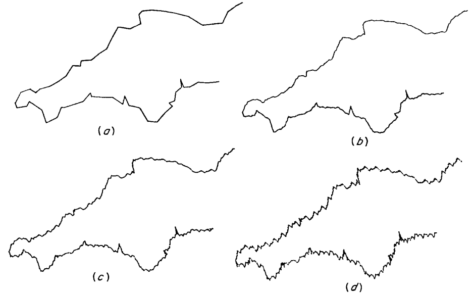
Figure 11.5 Fractal interpolation on the northern and southern halves of a map of South-West England, using the vertices of the polygon in figure (a) as data points. The dimensions of the self-affine curves fitted to these data points are (b) 1.1, (c) 1.2 and (d) 1.3
