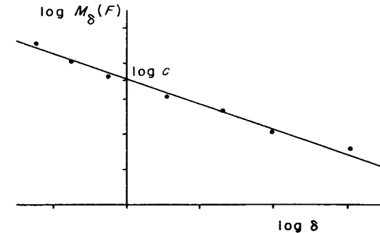
Figure 3.1 Empirical estimation of a dimension of a set F , on the power-law assumption M_\delta(F) \sim c\delta^{-s}
