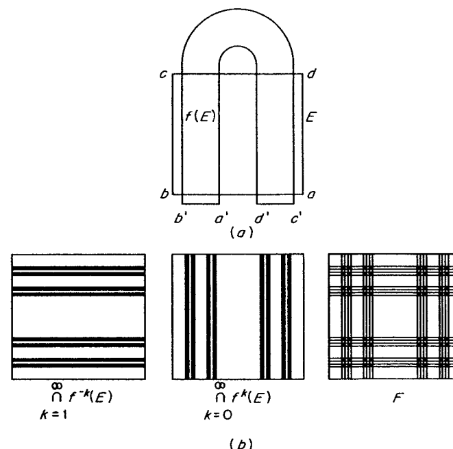
Figure 13.6 An alternative horseshoe map. (a) The square E is transformed so that the 'arch' and 'ends' of f(E) lie outside E . (b) The sets \bigcap_{k=1}^{\infty} f^{-k}(E) and \bigcap_{k=0}^{\infty} f^k(E) are both products of a Cantor set and a unit interval. Their intersection F is an unstable invariant set for f
