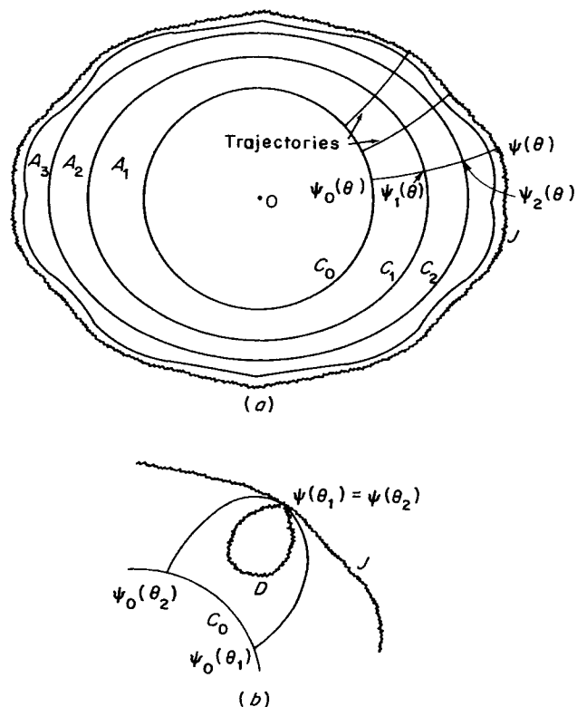
Figure 14.5 Proof of Theorem 14.16
