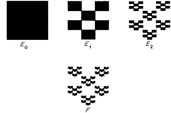
Figure 7.4 Construction of a self-affine set, \dim_H F = 1\frac{1}{2}
