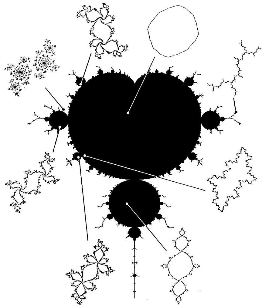
Figure 14.6 Julia sets J(f_c) for various points in the Mandelbrot set. The Julia sets are displayed in more detail in figure 14.7
