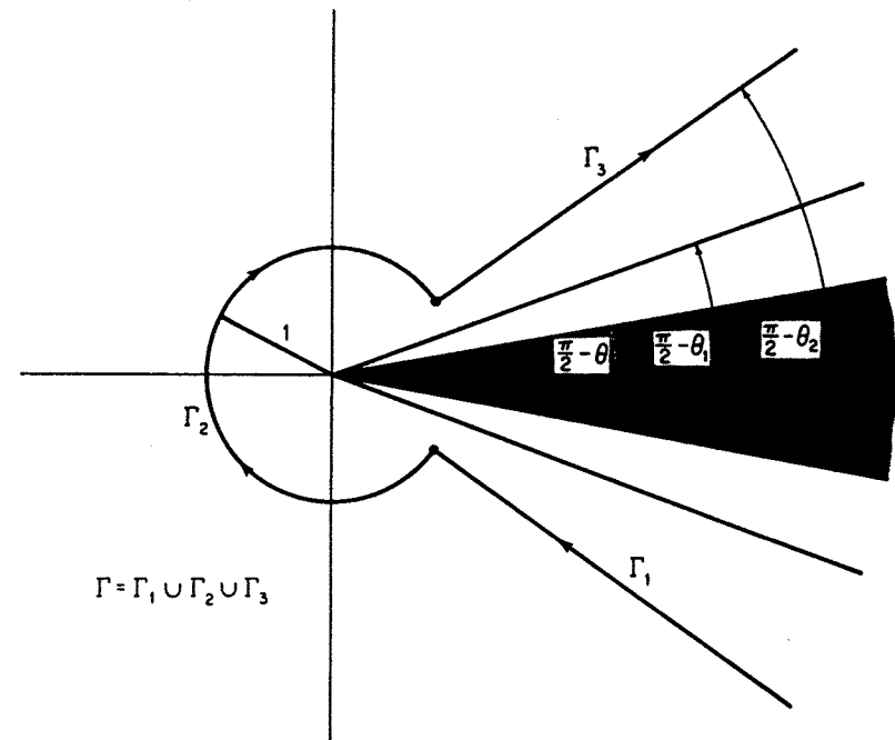
FIGURE X.5 The curve \Gamma .
