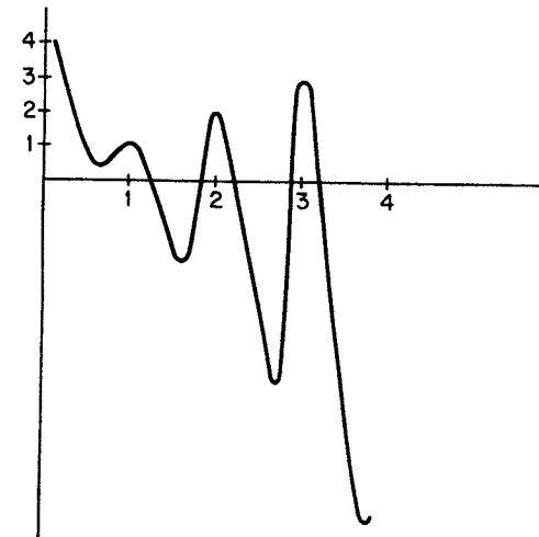
FIGURE X.3 The graph of V .
