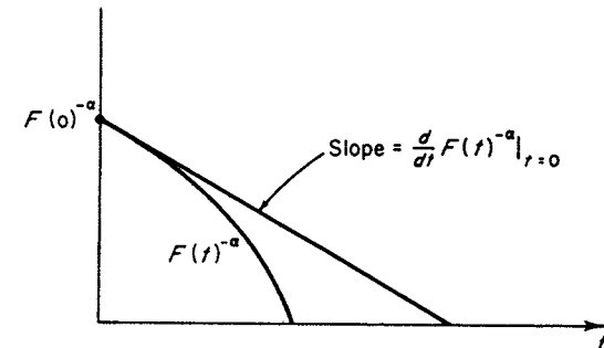
FIGURE X.8 The graph of F(t)^{-\alpha} .
