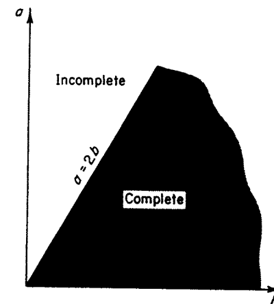
FIGURE X.10 Classical completeness for V_{ab} .
