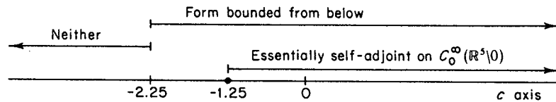
FIGURE X.4 The operator -\Delta + (c/r^2) when n = 5 .
