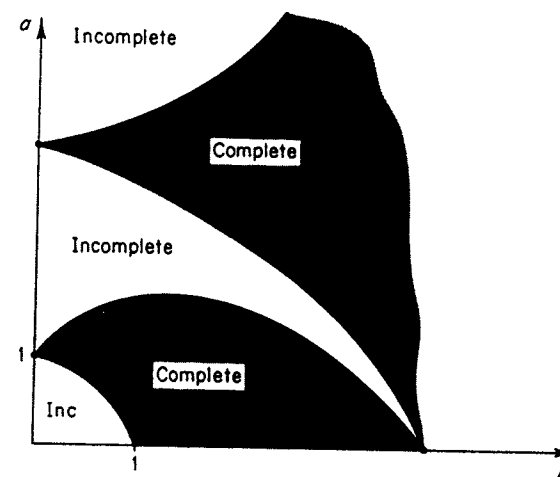
FIGURE X.9 Quantum-mechanical completeness for V_{ab} .
