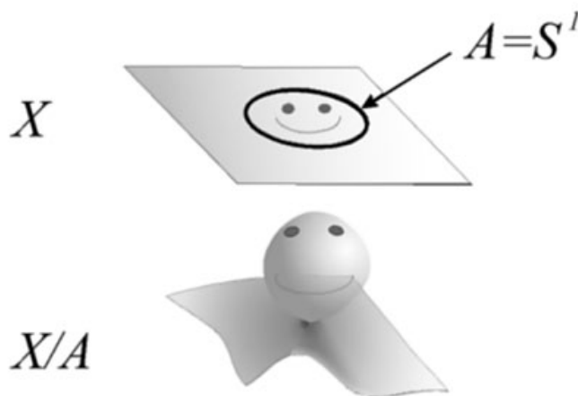
Figure 15.1: creation of a “hole”
