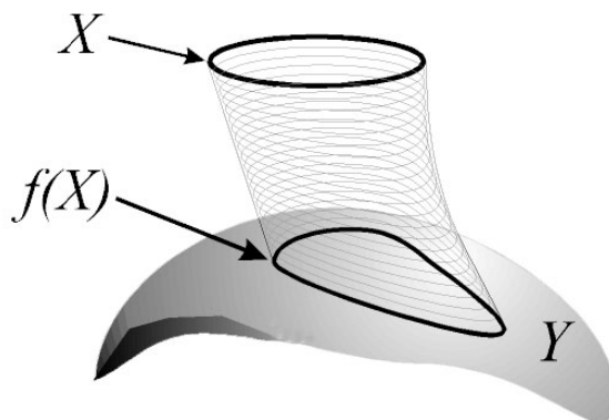
Figure 15.2: Mapping Cylinder
