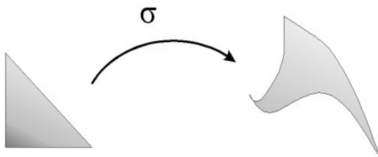
Figure 16.2: Singular 2-simplex
