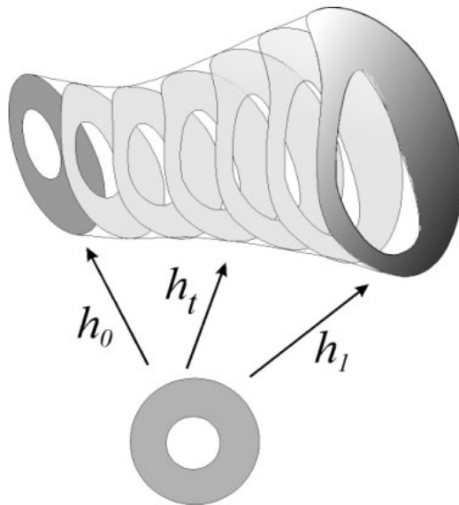
Homotopy as a family of maps.
