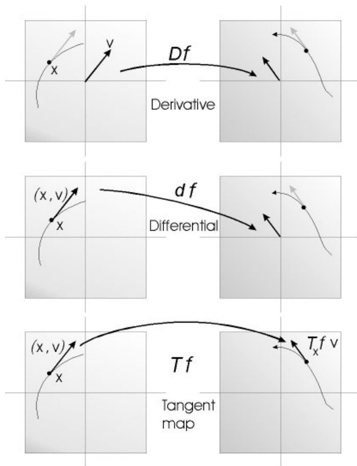
Figure 26.1: Versions of the “derivative” map.
