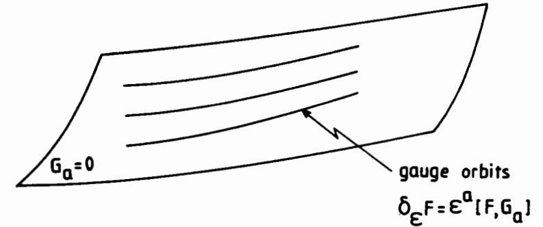
Figure 3: The first-class constraint functions G_a define not only the constraint surface \Sigma through G_a = 0 but also the gauge orbits through \delta_\epsilon F = \epsilon^a (X_a F) with X_a F \equiv [F, G_a] . The gauge orbits define the longitudinal directions. The longitudinal derivative d takes derivatives only along the longitudinal directions.
