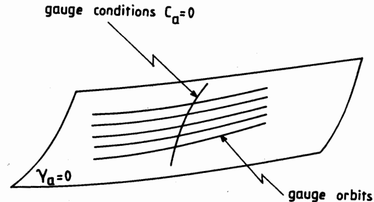
Figure 2: A good set of gauge conditions should determine a surface C_a = 0 that intersects the gauge orbits once and only once.
