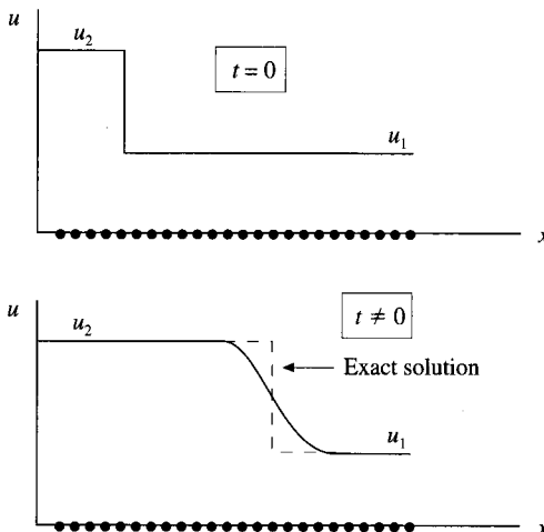
FIG. 11.4 Diffusive properties of the difference equation given by Eq. (11.55).
