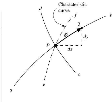
FIG. 3.2 Illustration of a characteristic curve.
