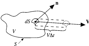
FIG. 2.4 Moving control volume used for the physical interpretation of the divergence of velocity.
