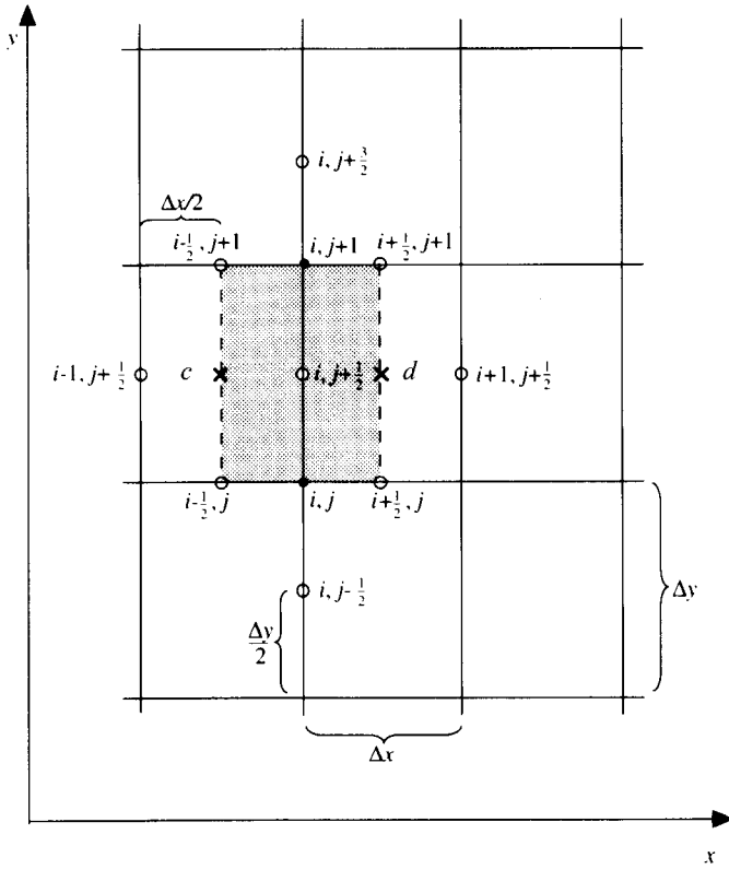
FIG. 6.17 Computational module for the y -momentum equation. The filled-in area is an effective control volume.
