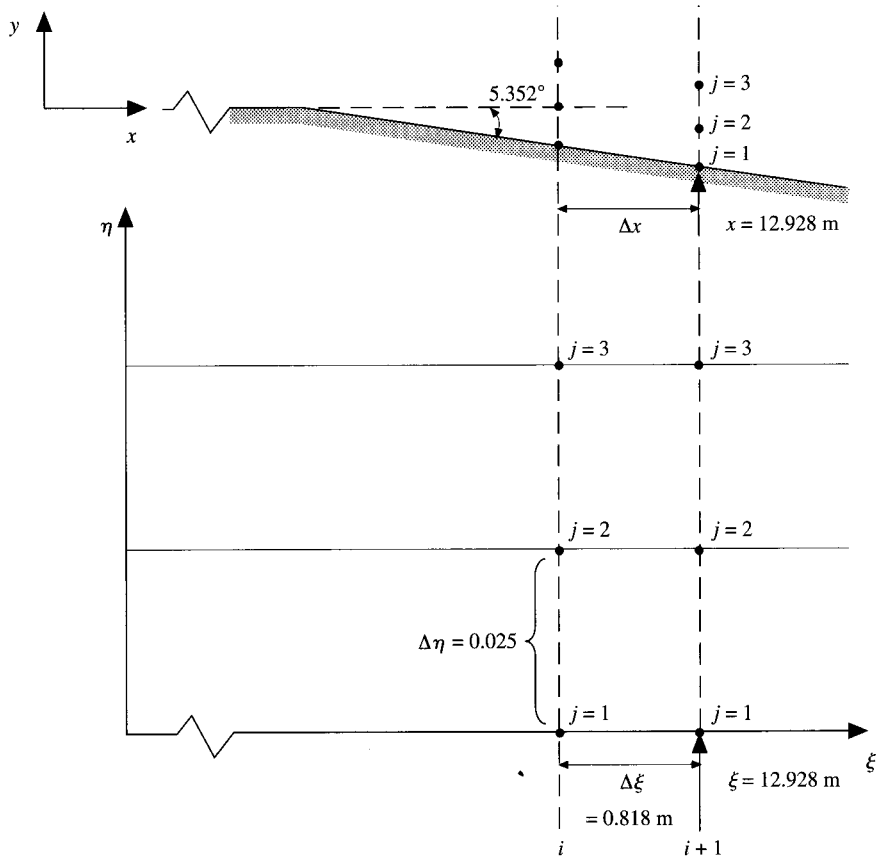
FIG. 8.7 Local grid adjacent to the wall at station x = \xi = 12.928 m.
