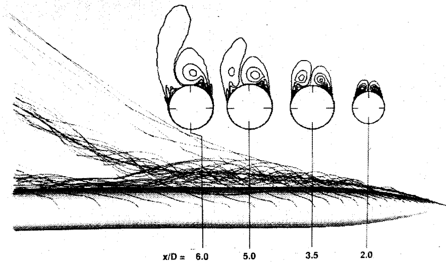
FIG. 6.26 Off-surface streamlines and helicity density contours around an ogive cylinder. M_\infty = 0.28 , angle of attack = 40^\circ , Reynolds number based on body diameter = 3 \times 10^6 . (From Ref. 71. Copyright © 1991, AIAA. Reprinted with permission.)
