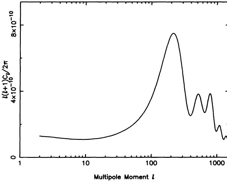
Figure A5.3 A typical prediction of cosmic microwave anisotropies, in this case for the Standard Cosmological Model. The predicted curve is calculated to better than one percent accuracy.
