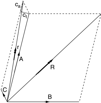
Figure 1.1 Vector addition by the parallelogram rule. Fields represented in magnitude and direction by the vectors A and B combine to give the resultant R. The resultant r of A and the smaller field C is approximately equal in length to the sum of A and the component c_a of C in the direction of A. The transverse component c_t rotates the resultant but has little effect on its magnitude.
