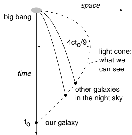
Figure 233 Speed and distance of remote galaxies
