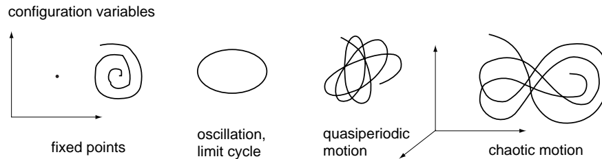
Figure 79 Examples of different types of motion in configuration space
