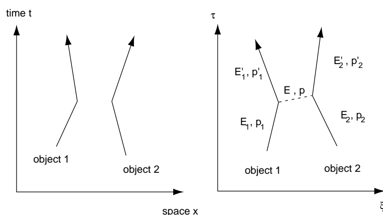
Figure 100 Space-time diagram of two interacting particles
