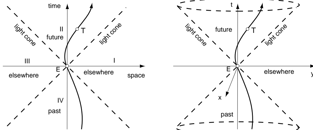
Figure 88 A space-time diagram of an object T seen from an inertial observer O in the case of one and of two spatial dimensions
