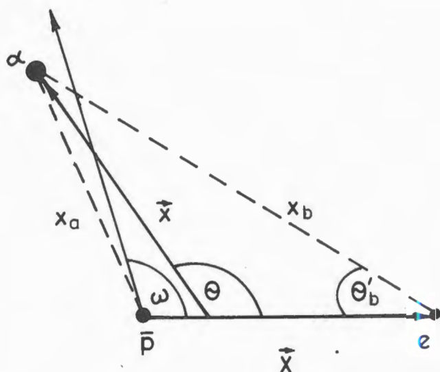
Figure. Three-body molecular Jacobi coordinates \mathbf{X} and \mathbf{x} (c-set), with \alpha -particle playing the role of the valence particle, form the reference configuration [ \tan(2\omega) = \mu x^2 \sin(2\theta) / (MX^2 + \mu x^2 \cos(2\theta)) ]. As \alpha -particle and \bar{p} are much more heavier than electron, the actual position of \mathbf{x} and the inertial tensor principal axis cannot be pictured properly, they practically coincide with x_a and \omega \approx \theta'_b . Two additional Jacobi-vector sets (a and b) are not pictured. They are defined as in our paper [8]
