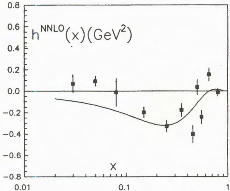
Figure. Higher-twist contributions from NNLO fit and the theoretical prediction for h(x) from [26]
