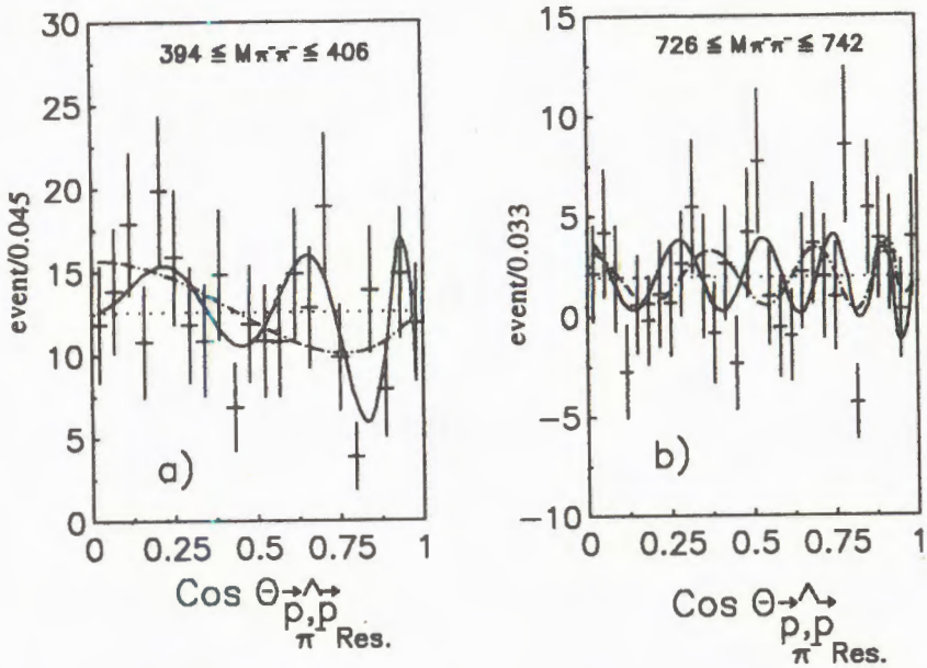
Fig.2. a) The distribution of \cos \Theta_{\vec{P}_{\pi^-}, \vec{P}_{Res}} for resonance at the mass of 397 MeV/c 2 and b) for resonance at the mass of 736 MeV/c 2 .
