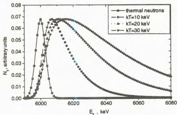
Fig. 2. The 6 MeV \gamma -line shapes registered by the Ge(Li)-detector for the capture of the neutrons from Maxwellian spectra, as well as thermal neutrons
