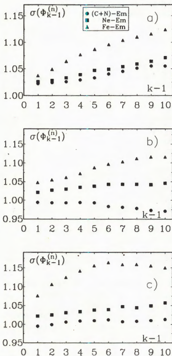
Fig.5. The \sigma(\Phi_{k-1}^{(n)}) vs. k for s -particles (a), g -particles (b) and b -particles (c) from nucleus-nucleus collisions. The spectator fragments of projectile nuclei are excluded from relativistic secondaries
