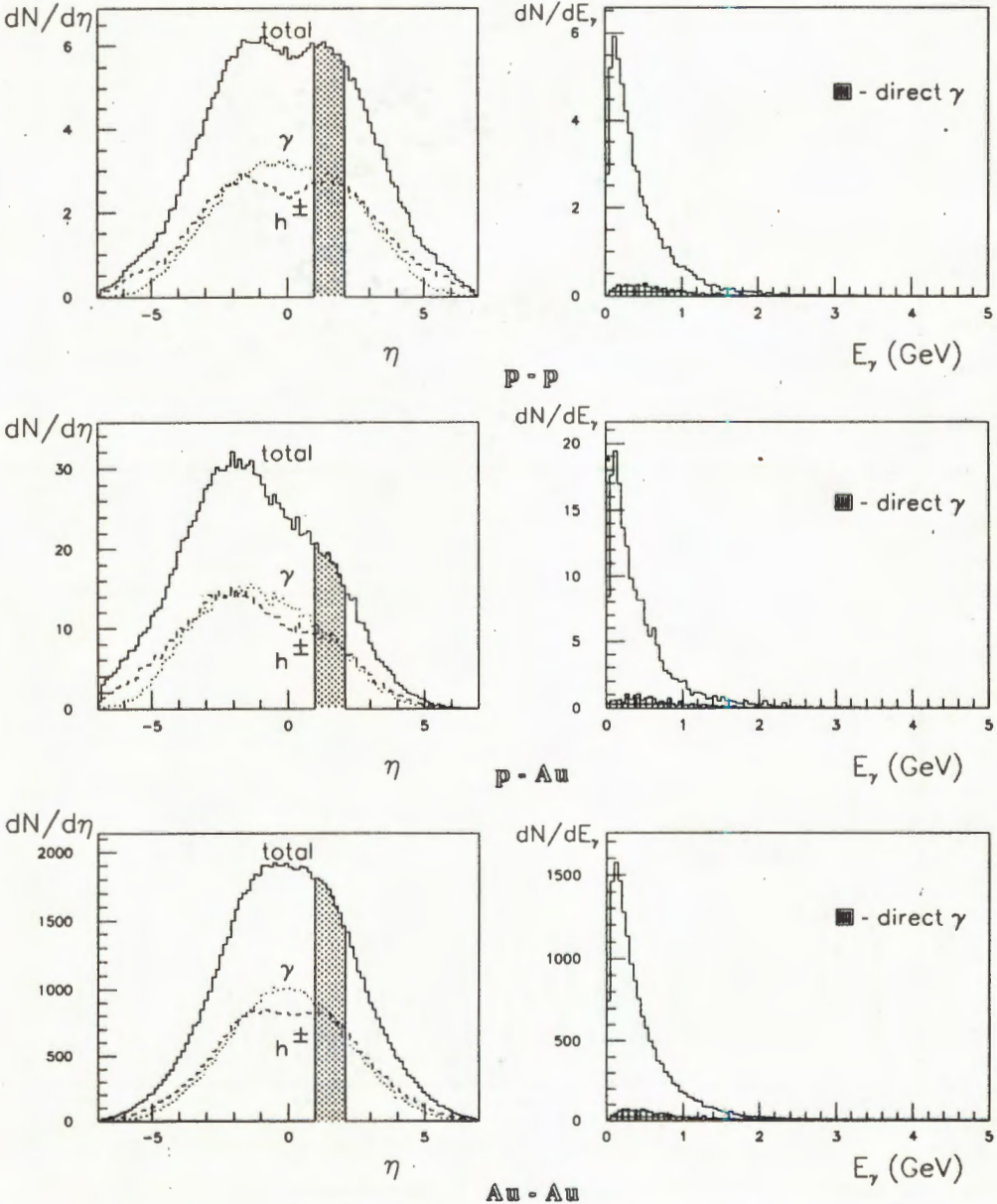
Fig.1. The pseudorapidity distribution of \gamma 's and charged hadrons in pp , p\text{Au} and \text{AuAu} collisions at 200 GeV/nucleon
