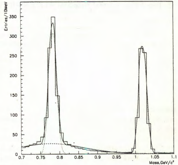
Fig.2. Effective mass distribution of pairs where both e^+ and e^- come from one of the resonances ( \rho^0 , \omega or \phi ). The curves are the results of Gaussian fits
