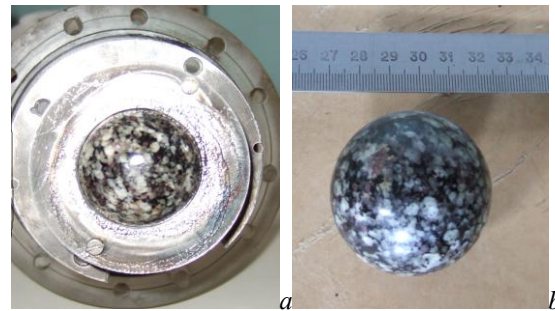
Fig. 1. Type of the experimental sample of granite, which is made in the form of a ball: and – a fixed accelerator target; b – perspective view
