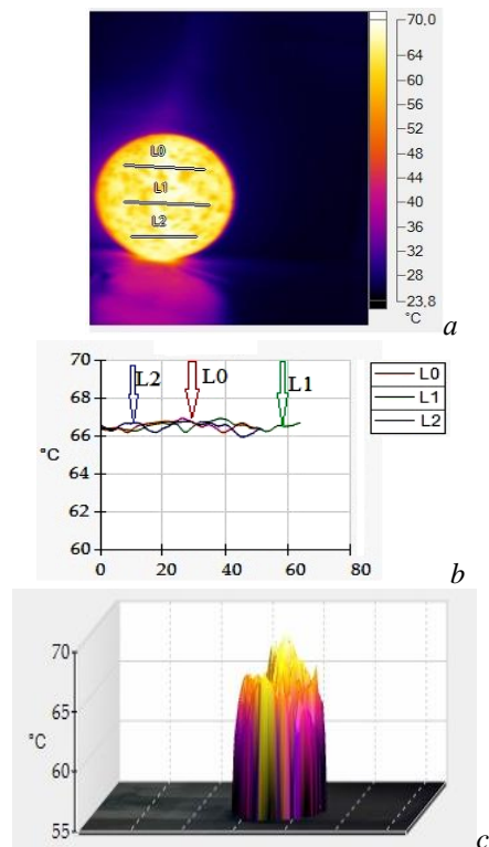
Fig. 4. The thermogram (a); graph (b), and 3D image (c) non-treated surface of the ball in the absence of moisture
