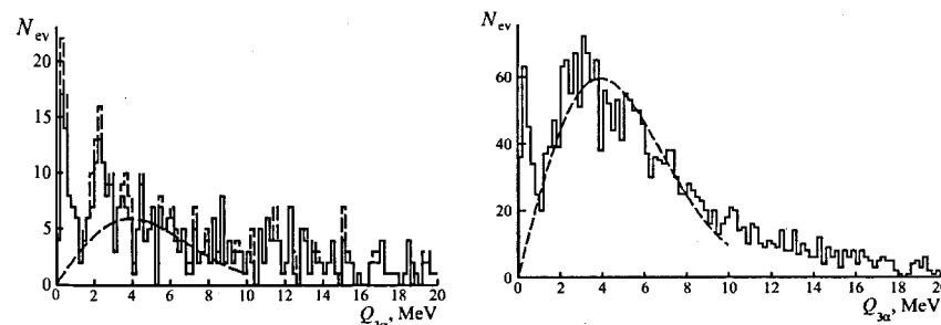
Fig. Distribution over invariant mass Q_{3\alpha} of \alpha -triples in dissociation of 12 C \rightarrow 3 \alpha GeV (left) and 3 \alpha combinations in "white" stars 16 O \rightarrow 4 \alpha at 3.65 A GeV (right).
