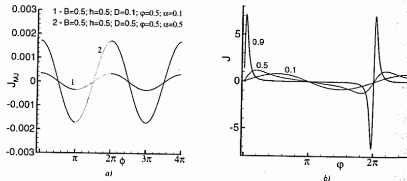
Fig. 1. a) Spin current as a function of magnetic field orientation, b) transformation of current-phase relation.
