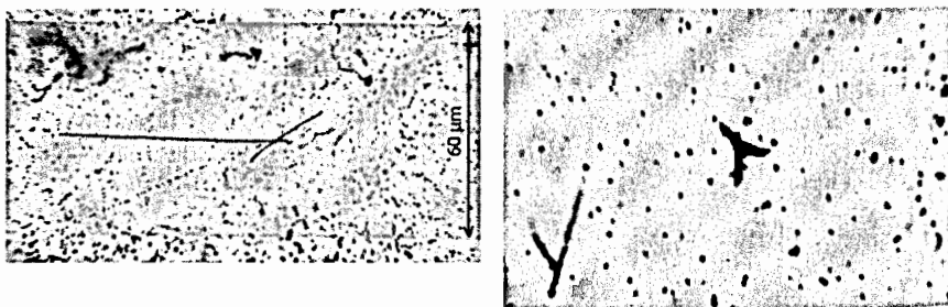
Fig. Macro photographs of hammer-like decay of the ^8\text{He} nucleus stopped in the nuclear track emulsion (left; superposed on a macro photograph of a human hair 60 \mu\text{m} thick) and Cf ternary fission (right).
