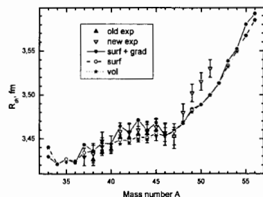
Fig.1 The impact of the different forms of pairing correlations (volume, surface, surface+gradient) on the charge radii. The experimental data are from [1].
