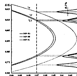
Fig. 1. Kinematics for the detection of multi-neutron membrane clusters on a beam of heavy ^{16}\text{O} ions.
