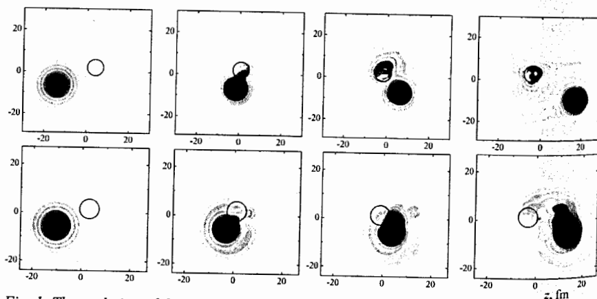
Fig. 1. The evolution of the probability density p(r,t) of external protons of the ^8\text{B} nucleus in its collision with the ^{28}\text{Si} nucleus (circle) at energy E_{\text{lab}} = 10 \text{ A MeV} (on top) and 64 \text{ A MeV} (below); the course of time corresponds to panels from left to right.
