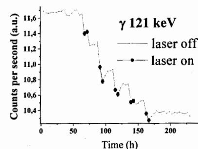
Fig.1. The change in the intensity of the gamma line 121 keV ^{152}\text{Eu} .
