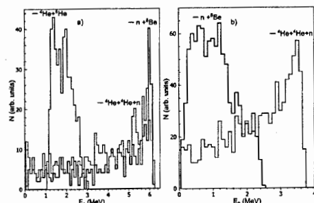
Fig. 1. Simulation of reactions ^9\text{Be}(d,d'n)X (a) and ^9\text{Be}(d,d'\alpha)X (b) for various breakup channels at deuteron beam energy of 15 MeV. (a) – Neutron spectrum from the breakup of E^* = 6.76 MeV level, \Theta_d = 30^\circ , \Theta_n = 20^\circ ; (b) – Alpha spectrum from the breakup of E^* = 3.05 MeV level, \Theta_d = 50^\circ , \Theta_\alpha = 55^\circ .
