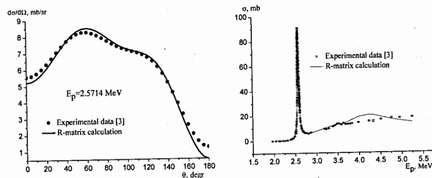
Fig.1. Description of differential and total ^9\text{Be}(p,\alpha_2)^6\text{Li}^* (3.563 MeV) reaction cross-sections.
