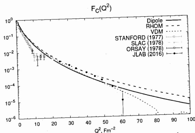
Fig. 1. Helium-3 form factors: Dipole - dipole fit, RHOM - relativistic harmonic oscillator model, VDM - vector dominance model.
