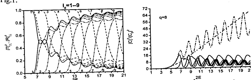
Fig. 1. Diagonal elements of the transmission |T|^2 and reflection |R|^2 matrices in first open channels ( i_0 = 1-9 ) (left), enhancement coefficient (C(E))^2 / (C_0(E))^2 , partial (solid), total (dash-dotted) and analytic (right) vs. collision energy E for similar charged particles ( q=6 , \gamma=1 ).
