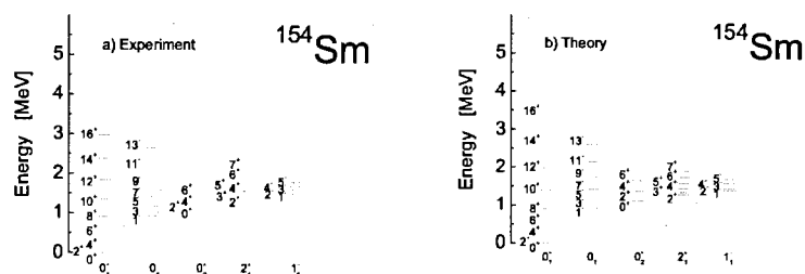
Fig. 1. Comparison of theoretical excitation energies ^{154}\text{Sm} with experiment.
