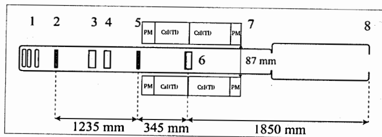
Fig. 1. Scheme of the detector setup "MULTI": 1 – degrader; 2 – active collimator AC1; 3 – 300 \mu\text{m} silicon pixel detector \Delta E "16X-16Y"; 4 – 380 \mu\text{m} silicon detector \Delta E_0 ; 5 – active collimator AC2; 6 – 243 \mu\text{m} active target Si – PIN; 7 – 12x CsI(Tl) gamma spectrometer; 8 – remote beam dump.
