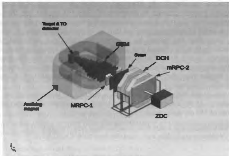
Fig. 1. The schematic view of the BM@N experiment.
