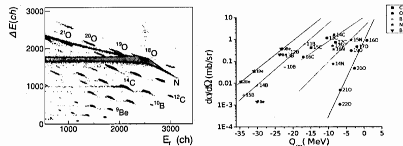
Fig.1 Left panel: Identification matrix \Delta E-E_r of the products of the ^{18}\text{O}(10\text{MeV/A}) + \text{Ta} reaction. Right panel: Q_{gg} systematic for the ^{18}\text{O}(10\text{ MeV/A}) + \text{Ta} reaction products.
