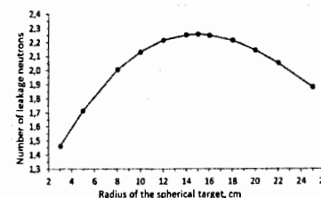
Fig. 1. The dependence of full fluence from ^{232}\text{Th} + ^{nat}\text{U} (50/50%) target thickness.
