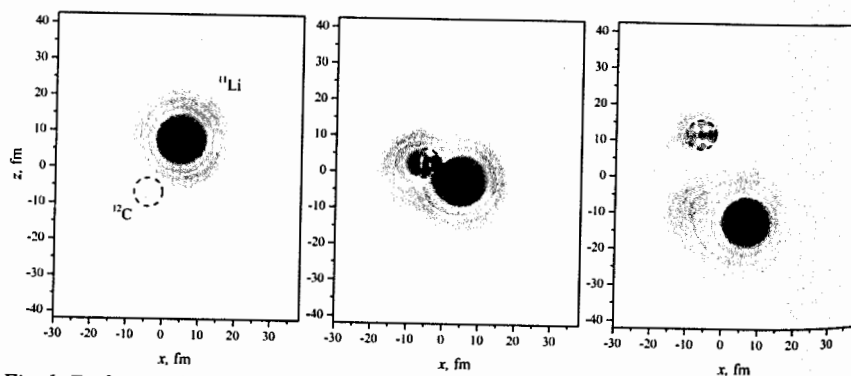
Fig. 1. Evolution of probability densities of external neutron of ^{11}\text{Li} in the collision with ^{12}\text{C} at E_{\text{c.m.}} = 18 MeV. Impact parameter b = 9 fm. Time scale from left to right. Dash circle is ^{12}\text{C} nucleus.
