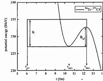
Figure 1. Synthesis box as a new approach to describe superheavy element decay.
