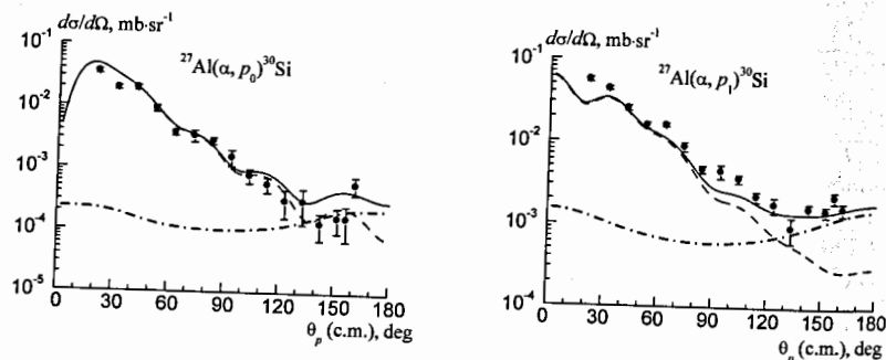
Fig. 1. Angular distributions of ^{27}\text{Al}(\alpha, p)^{30}\text{Si} reaction for transitions to the ground and first excited states of ^{30}\text{Si} . Presented calculation of CC (dashed line), CN (dotted-dash) and their incoherent sum (solid)
