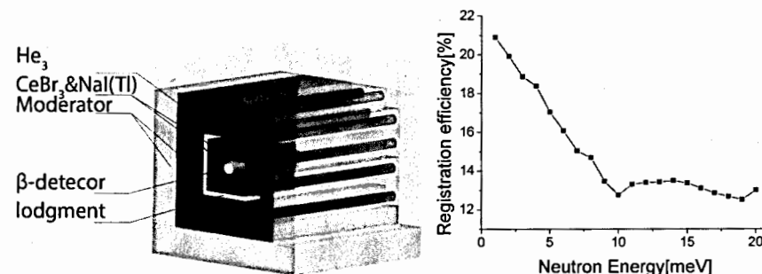
Fig. 1. Various geometries MULTI.
