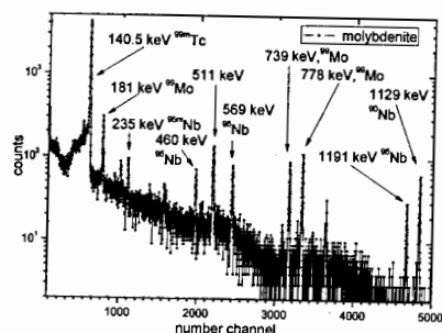
Fig. 1. The spectrum of molybdenite nanoparticles after irradiation by bremsstrahlung with E_{\text{max}} = 39 MeV
