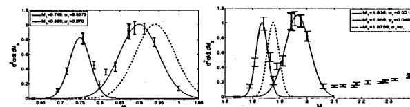
Fig.1. Effective mass ( \text{GeV}/c^2 ) distribution of particle X for d + d \rightarrow X + d reaction. Theoretical peaks for X = p and X = d are shown by dashed lines in the left and right pictures. Experimental data are taken from [1]. Parameters of their normal distribution interpolation shown by solid lines are also given.
