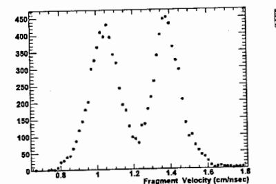
Fig. 2. The measured velocity spectrum of ^{252}\text{Cf} fission fragments.
