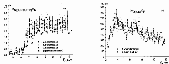
Fig.2. Cross-sections of {}^{14}\text{N}[(d,t) + (d,d+n)]{}^{13}\text{N} (a) and {}^{16}\text{O}(d,n){}^{17}\text{F} reactions (b).
