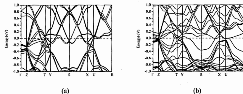
Fig. 1. Dispersion curve of \text{HTa}_{32}\text{P}_{32} (a) and \text{HTa}_{31}\text{P}_{32} (b). Circles indicate the Weyl points.
