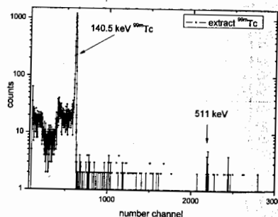
Fig. 2. The spectrum of extracted ^{99\text{m}}\text{Tc}
