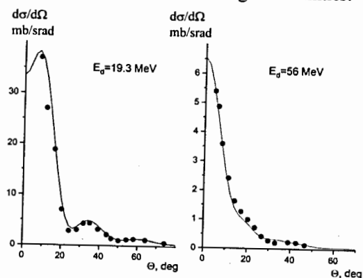
Fig. 1. Angular distributions of the ^{48}\text{Ca}(d,p)^{49}\text{Ca} reaction at E_d = 19.3 (left) and 56 (right) MeV found with the DOMP via DWBA approach.
