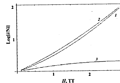
Fig. 2. Magnetic field dependence of yield ratio [i\text{Ni}] of ^{56}\text{Ni} and ^{44}\text{Ti} - 1, ^{48}\text{Cr} - 2, and ^{60}\text{Zn} - 3.
