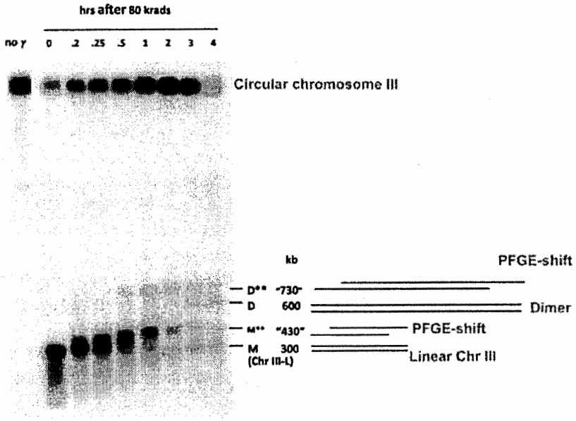
Figure 2 Single DSBs in circular chromosomes lead to linear molecules which exhibit PFGE-shift with time of incubation
