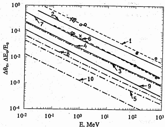
Fig.1. The maximum accuracies of the coincidence of the H^- ion and electron distributions at relative energy ( \Delta E_o/E_o , 1-5 curves) and angle ( \Delta\theta_o , 6-10) for different particle (1,6 - \diamond Kr[14], * Ne, CH_3Cl [15], \circ He[15, 16, 18], \times Ar[17, 19], \bullet C[24]) and photon ( \lambda = 10600\text{\AA} - 2,3,7,8; \lambda = 16300\text{\AA} - 4,5,9,10 [26-28]) targets versus ion energy.
