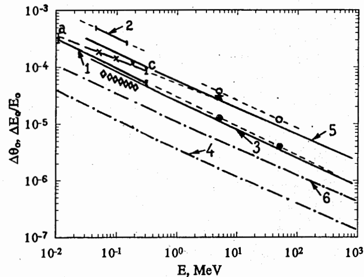
Fig.2. The maximum accuracies of the coincidence of the H^- ion and H^0 atom distributions at angle ( \Delta\theta_o \rightarrow 1,2,*, \times , \diamond - exp.; \bullet ,3,4 - theor.) and relative energy ( \Delta E_o/E_o \rightarrow 0,5,6 - theor.) for different particle (1 - He, Ar, H_2 , N_2 , CO_2 , Kr, Xe; * - K[22]; 2 - H_2 [21]; \bullet , \circ - C, Ar, Ne, He[25]) and photon ( \lambda = 10600\text{\AA} \rightarrow \times , \diamond [23], 3-6[28]) targets versus ion energy.
