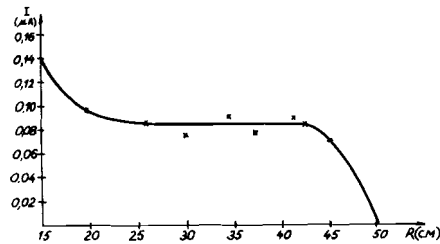
Fig. 4. Radial dependence of the proton current.
