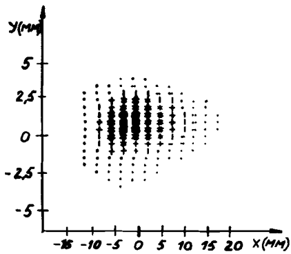
Fig. 4. Radial dependence of the proton current.
