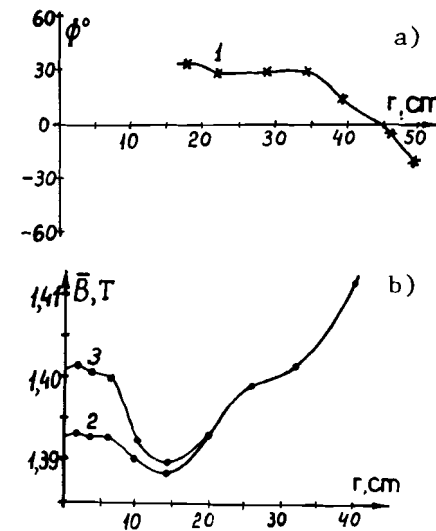
Fig. 5. (a) Phase motion of the proton bunch for field 5 (b) (2). (b) The shape of the magnetic field in the experiments: (2) optimal tuning for protons, (3) optimal tuning for simultaneous acceleration of two beams.
