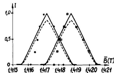
Fig. 2. Resonant curves for protons and H^- ions calculated on the assumption that I_{is} \sim V_{acc}^{3/2} (solid line), I_{is} \sim V_{acc}^3 (dashed line) and measured experimentally (circles and squares).
