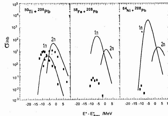
Fig. 8. The production cross section of elements 104, 108, 110 in cold fusion reactions (HI,1n). ■ - the experimental data obtained at the GSI, the lines are results of calculations within the framework of the statistical model [8].
