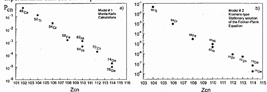
Fig. 7. The probability of complete fusion P_{cn} in the cold fusion reactions (HI,1n): a) the Monte-Carlo calculations are used, b) the Kramers type stationary solution to the Fokker-Planck equation is used.
