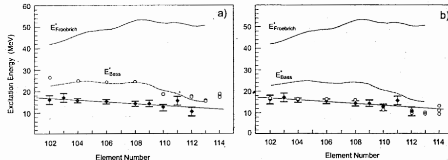
Fig. 6. The minimal excitation energy of the compound nuclei of 102-114 elements in cold fusion reactions (HI,1n). ♦ - the experimental data, ○ - the calculated data according to the DNS-concept: a) the deformation of the heavy nucleus of the DNS is taken into account, b) the deformation of the heavy and light nuclei of the DNS is taken into account.
