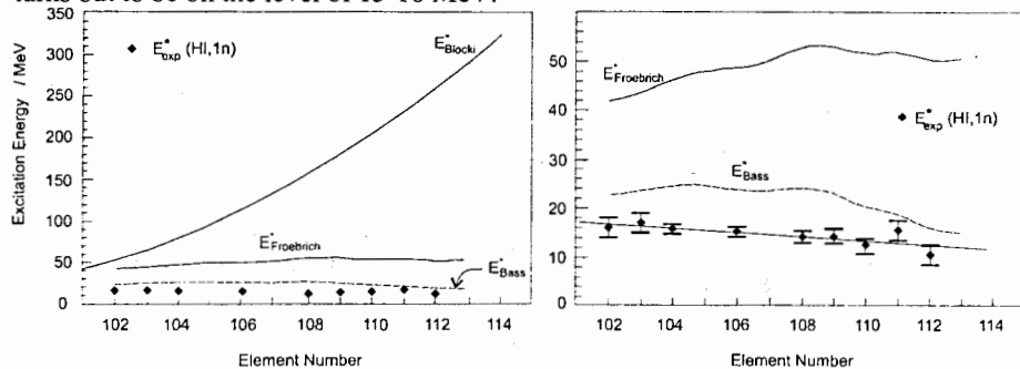
Fig. 4. The minimal excitation energy of the compound nuclei of the 102-112 elements which have been synthesized in cold fusion reactions (HI,1n). ♦ - the experimental data, the solid lines present the results of calculations within the framework of the MDM and the surface friction model, the dashed line indicates the compound nucleus excitation energy in the collision when kinetic energy is equal to the Bass barrier [5].
