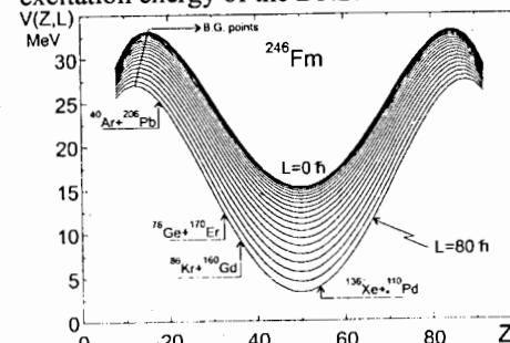
Fig. 2. Potential energy of the DNS which is formed in four reactions with the same compound nucleus ^{246}\text{Fm} . Z is the atomic number of one of the DNS nuclei.
