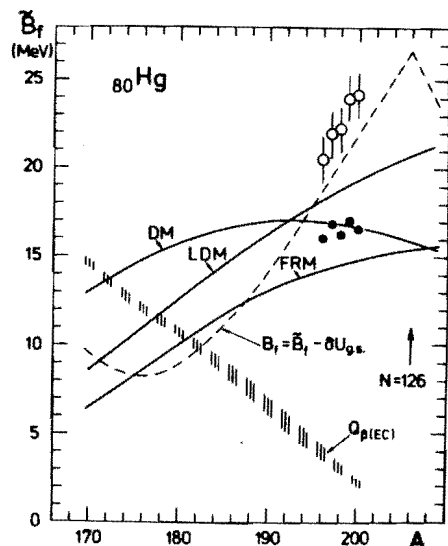
Fig. 1. The isospin dependence of the macroscopic part \tilde{B}_f of the fission barrier heights for Hg isotopes, as predicted by the droplet model of Myers (DM) 15/ , the liquid drop model of Myers and Swiatecki (LDM) 16/ , and the finite range model of Sierk (FRM) 12/ . The dashed curve shows the fission barriers B_f = \tilde{B}_f - \delta U_{g.s.} composed of the \tilde{B}_f values by Sierk 12/ and of the ground-state microscopic corrections \delta U_{g.s.} by Möller and Nix 17/ ; note that around ^{180}\text{Hg} the \delta U_{g.s.} corrections are small. The open circles represent the empirical fission barrier heights obtained in ref. 19/ from statistical-model analyses of the measured excitation functions for fission induced by light charged particles with A \leq 4 ; the closed circles show the macroscopic barrier heights \tilde{B}_f obtained by removing the calculated \delta U_{g.s.} corrections of Möller and Nix 17/ from the empirical B_f values. The triplets of vertical bars drawn for each even A outline, according to the mass tables 16-8/ , the "corridor" of the Q_{\beta^+}(EC) values for the odd-odd Tl isotopes; the bar heights thus reflect a scatter of the Q_{\beta^+}(EC) predictions.
