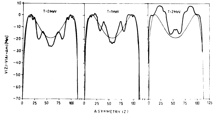
Fig.4. Potential energy V_Z of the system ^{283}_{113} as a function of the asymmetry parameter Z for three values of the nuclear temperature T = 0, 1 and 2 MeV. The thick and thin curves show the results obtained taking and without taking the shell effects into account, respectively.
