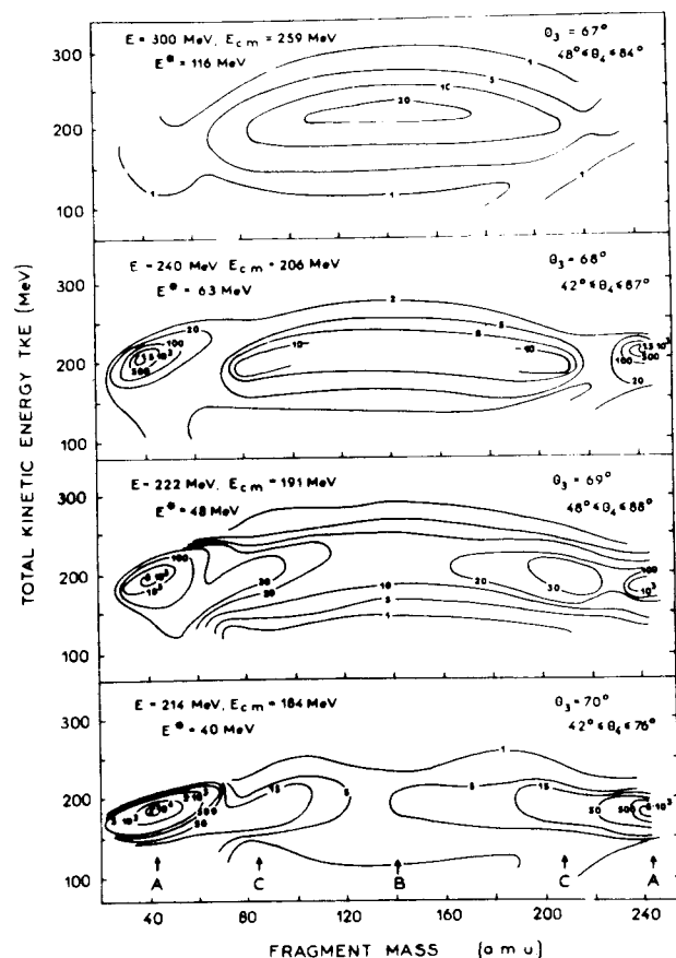
Fig.1. Total c.m. kinetic energy vs fragment mass contour diagrams for the system ^{40}\text{Ar} + ^{243}\text{Am} at four different values of bombarding energy.
