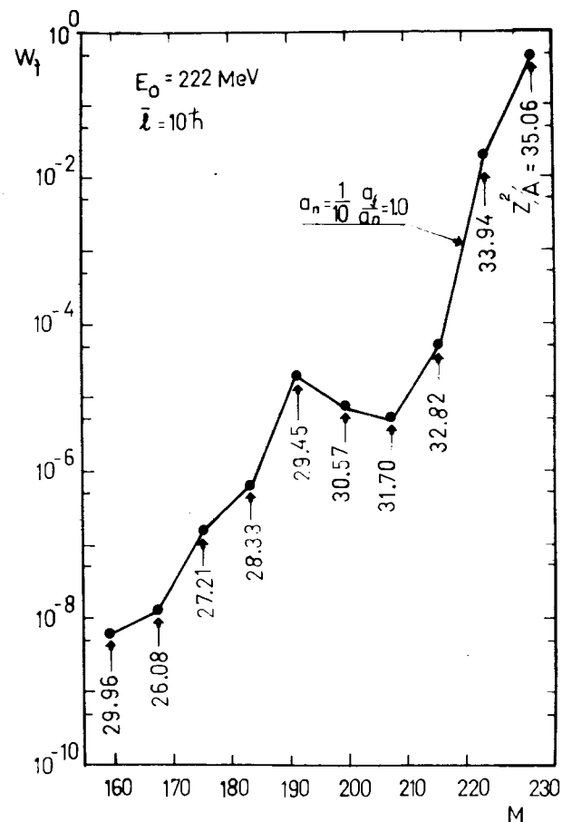
Fig.3. Calculated fission probabilities of the heavy nuclei produced in the reaction ^{40}\text{Ar} + ^{243}\text{Am} , as a function of mass.
