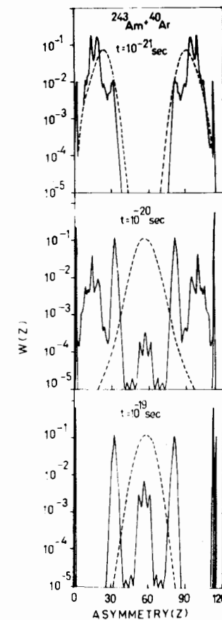
Fig.5. Calculated probability distributions W(Z) for three values of the diffusion time t = 10^{-21}, 10^{-20} and 10^{-19} sec in the case of T = 1 MeV. The full and dashed curves show the results obtained taking and without taking the shell effects into account, respectively.
