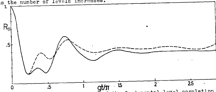
Figure 2. Short-time evolution of the fundamental level population R_{11}(t) for the four-level atom (solid line, g_1 = g_2 = g_3 = g , \bar{n}_1^0 = 5 , \bar{n}_2^0 = 0 , \bar{n}_3^0 = 1 ) and the three-level atom in the ladder configuration (broken line, g_1 = g_2 = g , g_3 = 0 , \bar{n}_1^0 = 5 , \bar{n}_3^0 = 1 ).
