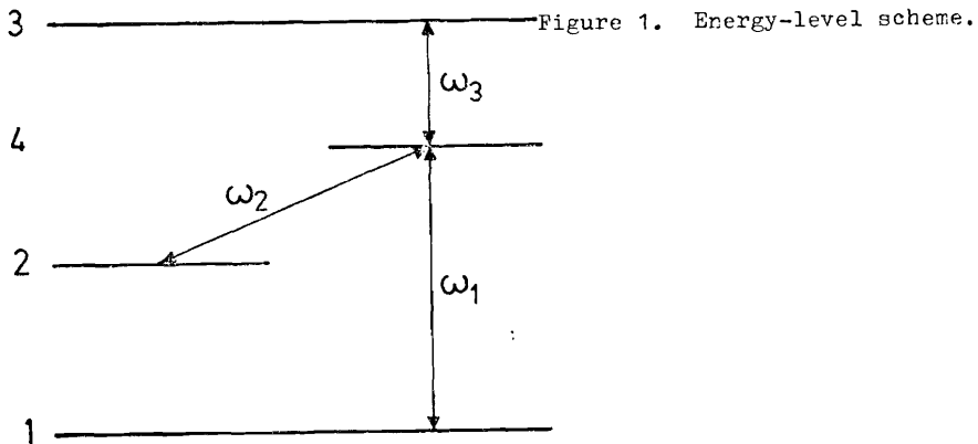
Figure 1. Energy-level scheme.
