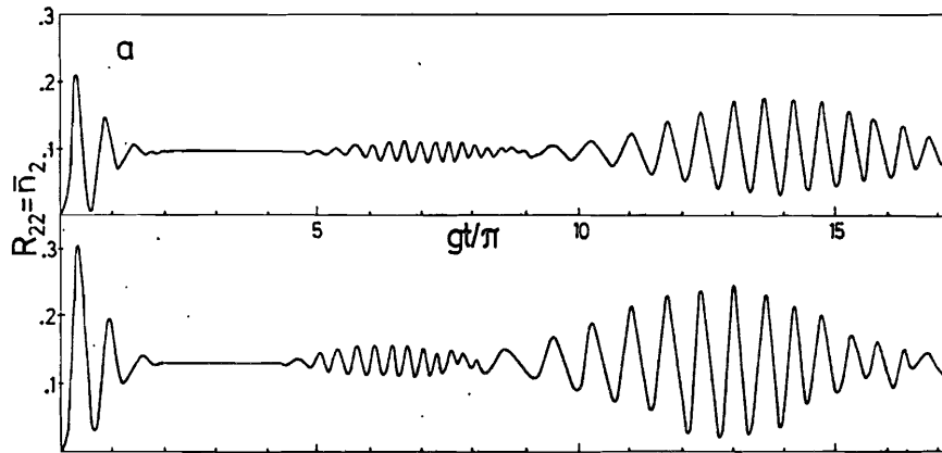
Figure 4. The time-dependence of the level 2 population: a/ the four-level atom ( g_1 = g_2 = g_3 = g , \bar{n}_1^0 = 10 , \bar{n}_2^0 = 0 , \bar{n}_3^0 = 2 ), b/ the three-level atom in the lambda configuration ( g_1 = g_2 = g , g_3 = 0 , \bar{n}_1^0 = 10 , \bar{n}_2^0 = 0 ).
