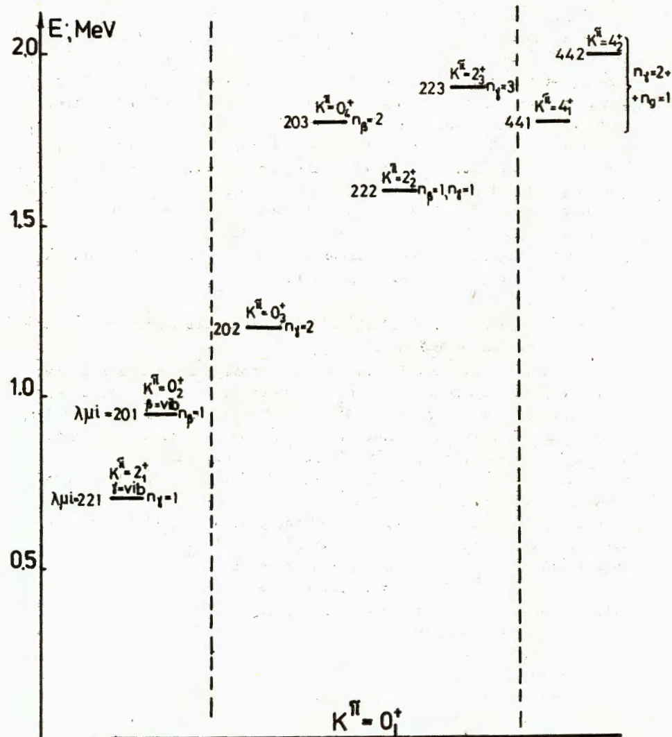
Scheme of nonrotational states of deformed nuclei with K_n^+ = 2_1^+, 0_2^+, 0_3^+, 0_4^+, 2_2^+, 2_3^+, 4_1^+ and 4_2^+ . For each level the dominating components are shown: on the left by the QPM and on the right by the IBM.
