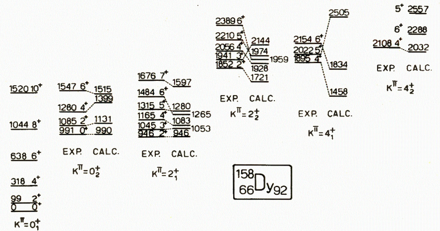
Fig.3. Calculated and experimental rotational positive parity bands in ^{158}\text{Dy} . Experimental data taken from /12/.
