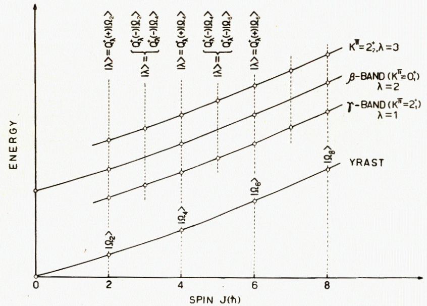
Fig.1. Scheme of the interpretation of the one-phonon states near the yrast line in RPA + SCCM method for low-spin region.
