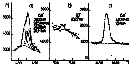
Fig. 2. Examples of fitting of the peaks.
