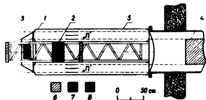
Fig. 1. Experimental arrangement.
