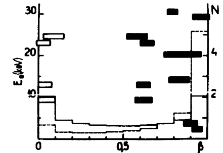
Fig. 3. \beta -distribution. N - relates to histograms and indicates the number of resonances (from 10 resonances) corresponding to the interval of width 0.1.
