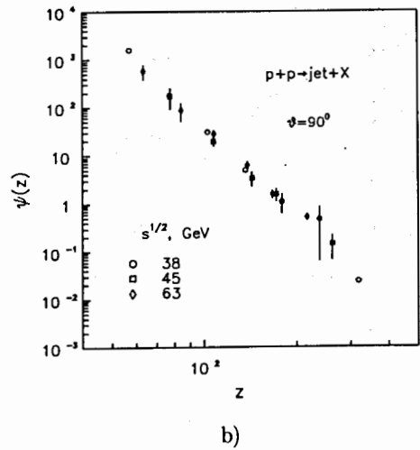
Figure 9. (a) The dependence of the inclusive cross section of jet production in pp collisions at \sqrt{s} = 38.8, 45 and 63 \text{GeV}/c and central rapidity range on transverse momentum q_T . The experimental data on the cross section obtained by the AFS and E557 collaborations are taken from Refs. [3, 23]. (b) The corresponding scaling function \psi(z) .
