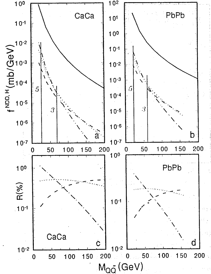
Figure 4. The same as in Fig. 3 only for CaCa non-coherent scattering at \sqrt{s_0} = 6.3TeV per nucleon (a,c) and PbPb at \sqrt{s_0} = 5.5TeV per nucleon (b,d). Factor (13) is not taken into account.
