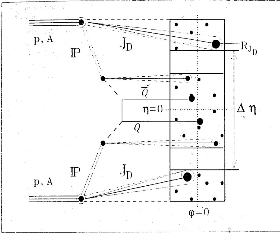
Figure 1. Schematic representation of heavy quark - antiquark production in Double Diffractive scattering (4) using the hypothesis of factorization in the plane of azimuthal angle ( \phi ) and pseudorapidity ( \eta ). Projectiles (protons - p or nuclei - A ) emit Pomerons ( IP ) and escape as diffractive jets ( J_D ), the interval between which ( \Delta\eta ) is a "rapidity gap". The quark - antiquark pair ( Q\bar{Q} ) is produced from the hard (QCD) interaction of both Pomerons. The radius of the diffractive cones in ( \eta, \phi ) is taken equal to R_{J_D} \simeq 0.7 .
