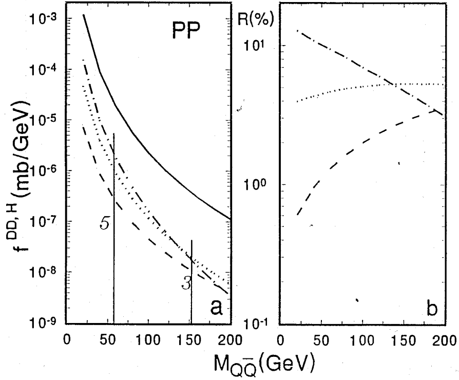
Figure 3. Dependence of (a) the differential cross section of quark - antiquark pair production f^{DD,H}(mb/GeV) = \frac{d^3\sigma^{DD,H}}{dM_{Q\bar{Q}}d\eta_Qd\eta_{\bar{Q}}} at \eta_Q = \eta_{\bar{Q}} = 0 (14) and (b) the ratio R(\%) = f^{DD}/f^H (15) on the invariant mass of quark pair M_{Q\bar{Q}}(GeV) for the chosen models of Pomeron: (7) - dot-dashed lines, (8) - dashed lines, (9) - dotted lines, solid line is for hard (QCD) process. \sqrt{s_0} = 14TeV , factor (13) is not taken into account. Upper limits on M_{Q\bar{Q}} for \Delta\eta = 3 and 5 are denoted by upright lines.
