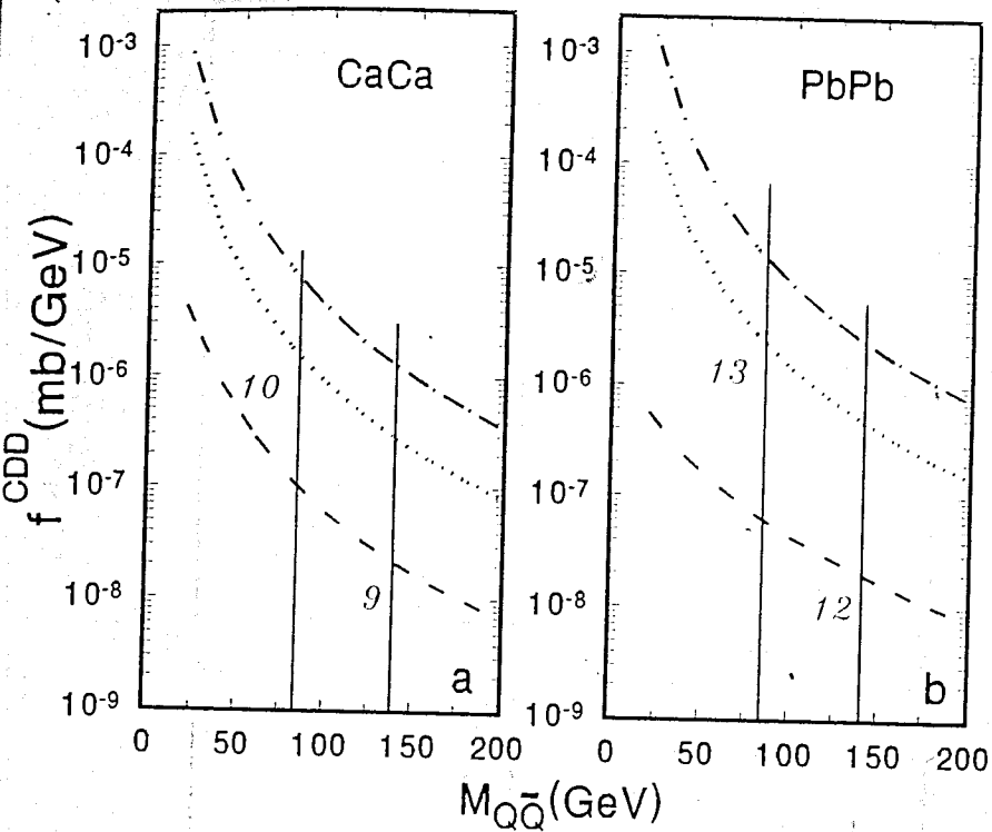
Figure 5. Dependence of the differential cross section f^{CDD}(mb/GeV) (14) of Q\bar{Q} production in the coherent double diffractive scattering of CaCa (a) and PbPb (b) on the invariant mass of pair M_{Q\bar{Q}}(GeV) at \eta_Q = \eta_{\bar{Q}} = 0 for the chosen models of Pomeron. The designations are the same as in the previous figures. Factor (13) is not taken into account. The upper limits on M_{Q\bar{Q}} are denoted for \Delta\eta = 9, 10 ( CaCa ) and \Delta\eta = 12, 13 ( PbPb ) by straight lines.
