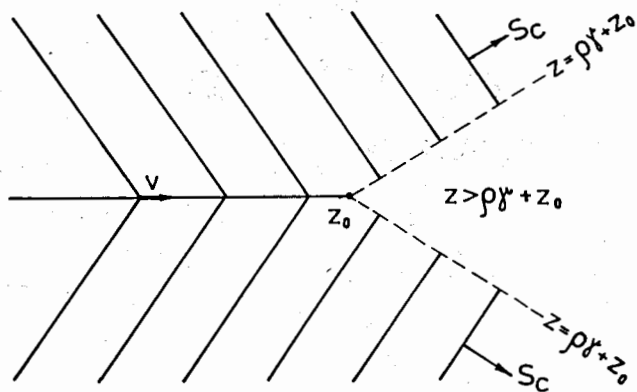
Fig. 3 The superluminal motion ends by the rest state at z = z_0 . In the region z > \rho\gamma_n + z_0 the observer sees no field up to some moment, when the shock bremsstrahlung wave reaches him. Later he sees the EMF of the resting charge and the EMF from one retarded position of the charge. In the region z < \rho\gamma_n + z_0 the EMF equals zero up to some moment when the Čerenkov shock wave reaches the observer. After that he sees EMF from two retarded positions of the charge up to the moment when the bremsstrahlung shock wave reaches him. Later, the observer sees simultaneously the field of the resting charge and that of the retarded positions of the charge.
