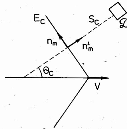
Fig.1 Čerenkov shock wave propagating in the infinite medium. There is no EMF in front of the Mach cone. Behind it there is EMF of the moving charge. At the Mach cone itself there are singular electric E and magnetic H fields. The latter having only the \phi component is perpendicular to the plane of figure.
