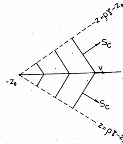
Fig.2. The superluminal motion of the charge begins from the rest state at z = -z_0 . In the z < \rho \gamma_n - z_0 region the observer sees (consecutively in time) the EMF of the resting charge, the bremsstrahlung shock wave and the EMF of the moving charge. There is no Čerenkov radiation in this space region. In the z > \rho \gamma_n - z_0 region the observer consecutively sees the EMF of the resting charge, the Čerenkov shock wave, the EMF from two retarded positions of the charge, the bremsstrahlung and the EMF from the moving away retarded position of the charge.
