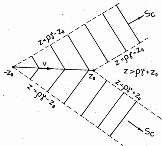
Fig. 4. The superluminal motion begins from the rest state at the point z = -z_0 and ends by the rest state at the point z = z_0 . For the finite distances the space-time distribution of EMF is rather complicated (see the text). The distant observer will see the following space-time picture. In the region z < \rho\gamma_n - z_0 he detects the bremsstrahlung shock wave from the z = -z_0 point first and from the z = z_0 point later. In the z > \rho\gamma_n + z_0 region these waves arrive in the reverse order. In the \rho\gamma - z_0 < z < (\rho^2\gamma_n^2 + z_0^2/\beta_n^2)^{1/2} region the observer consecutively detects the Čerenkov shock wave, bremsstrahlung from the z = -z_0 point and bremsstrahlung from the z = z_0 point. In the region (\rho^2\gamma_n^2 + z_0^2/\beta_n^2)^{1/2} < z < \rho\gamma_n + z_0 the latter two waves arrive in the reverse order.
