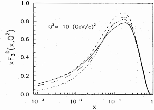
Figure 2. Deep-inelastic deuteron structure function x F_3^D(x, Q^2) . Theoretical results have been obtained with the parton distributions taken from: - - - [8], - · - [19], - - - [20], — [21].
