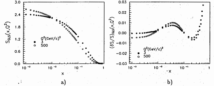
Figure 4. The Gross-Llewellyn Smith integral S_G(x, Q^2) and the correction (\delta S/S)_{GLS} due to the nuclear effect.
