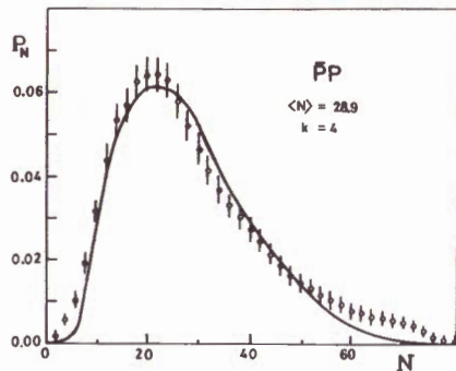
Fig.1. The multiplicity distribution of charged particles produced in antiproton-proton collisions at \sqrt{s} = 540 GeV. The data are taken from Ref. /10/ . The solid line is found from formula (5) with k = 4 .
