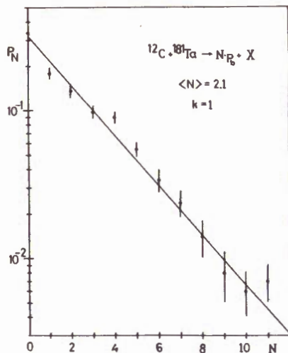
Fig.3. The multiplicity distribution of protons with momentum greater than 240 MeV/c emitted in the backward (in LAB) hemisphere for ^{12}\text{C}-^{181}\text{Ta} collisions at a momentum of 4.2 GeV/c per nucleon. The data are taken from Ref. /12/. The solid line corresponds to the geometrical distribution (3).
