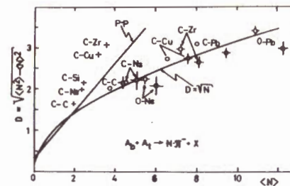
Fig.2. The dispersion versus the average number of negative pions produced in nucleus-nucleus collisions at a momentum 4.5 GeV/c per nucleon. Crosses - inelastic collisions, circles - central collisions. The full and open circles correspond to different central triggers, for details see Ref. /11/ . The straight line corresponding to multiplicity distributions for proton-proton inelastic collisions is found according to Wróblewski formula /2/ .
