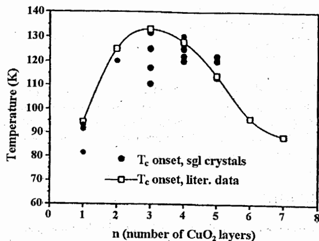
Fig. 1: Dependence of the superconducting critical temperature on number of layers n from Ref. [19].
