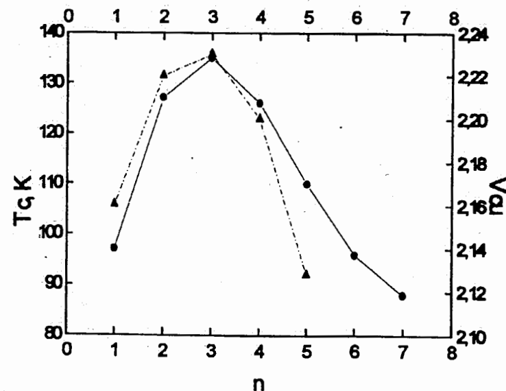
Fig. 3: Dependence of the superconducting critical temperature and copper valence on number of layers n according to data from Table 1. Full line is the critical temperature and dashed line is valence.
