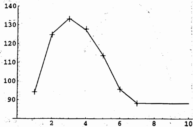
Fig. 5: Dependence of superconducting critical temperature T_c(n) with m = 3 fixed. Parameters: T_a^0 = 189.1 ; T_b^0 = 88.1 ; h_1 = 0.313 ; h_2 = 0.504 .
