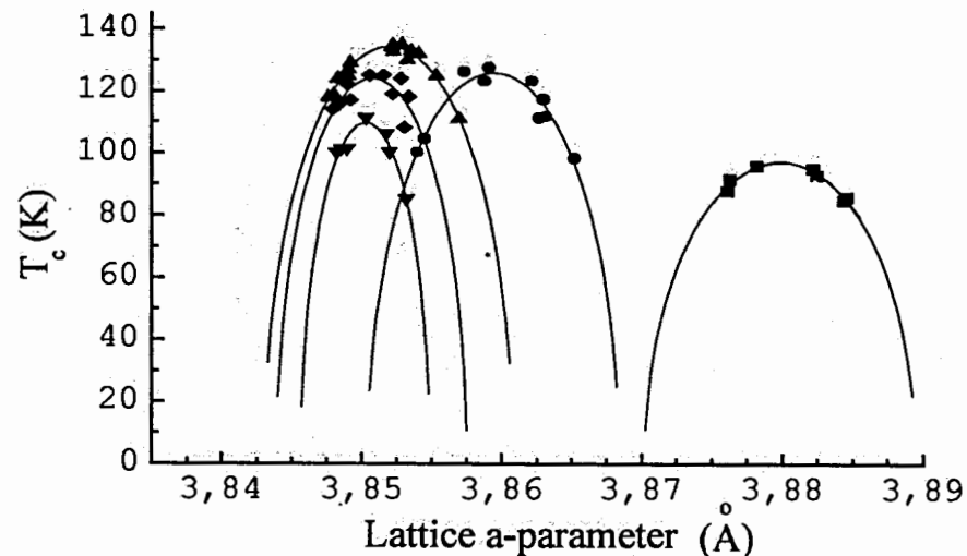
Fig. 2: Dependence of the superconducting critical temperature on lattice distance a for n = 1 - 5 . \square - n = 1 ; \bullet - n = 2 ; \triangle - n = 3 ; \diamond - n = 4 ; \nabla - n = 5 ; (c.f. [8])
