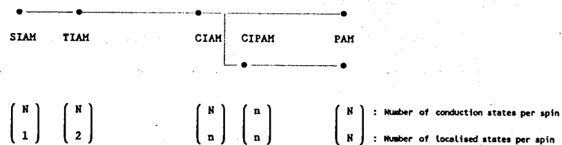
FIG. 1. The hierarchy of the Anderson models (the numbers are given in the case of 's' orbitals with n \leq N ). For a detailed presentation of the CIPAM, see also Ref. 65.
