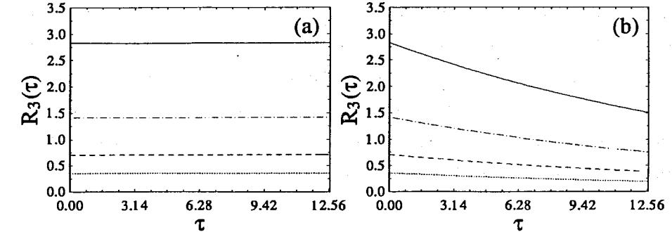
FIG. 7. Evolution of R_3(\tau) , for \eta = \pi/8 .
