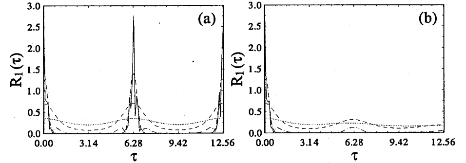
FIG. 5. Same as Fig. 4, but for \eta = \pi/8 .
