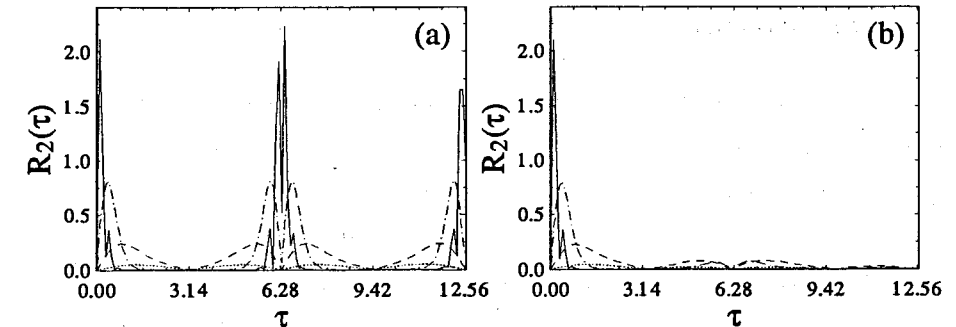
FIG. 6. Evolution of R_2(\tau) , for \eta = \pi/8 .
