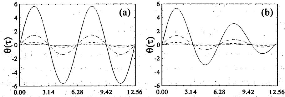
FIG. 1. Evolution of the azimuth \theta(\tau) for \eta = \pi/8 . The other parameters are taken the same for all the figures, and they are: d = 1 , |\alpha|^2 = 0.25 (dotted line), 1 (dashed line), 4 (dashed-dotted line), 16 (solid line). Figure (a) is for \lambda = 0 , and (b) for \lambda = 0.1 .
