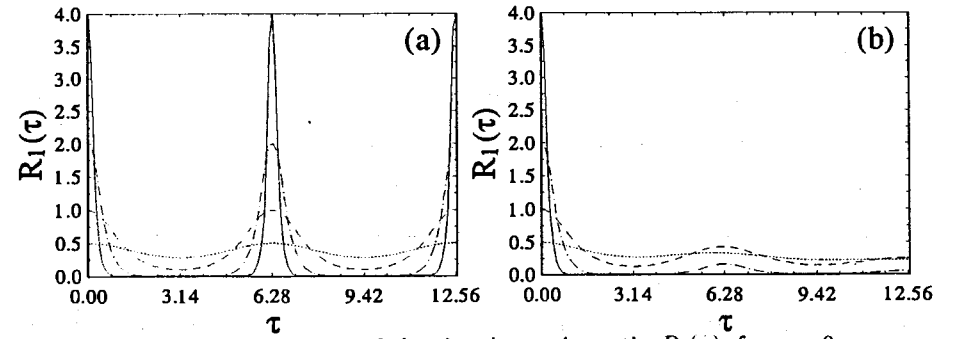
FIG. 4. Evolution of the signal-to-noise ratio R_1(\tau) , for \eta = 0 .
