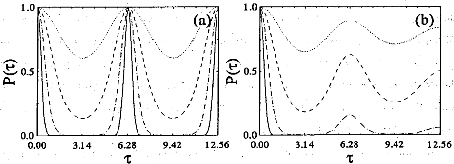
FIG. 3. Evolution of the degree of polarization P(\tau) , for \eta = 0 .
