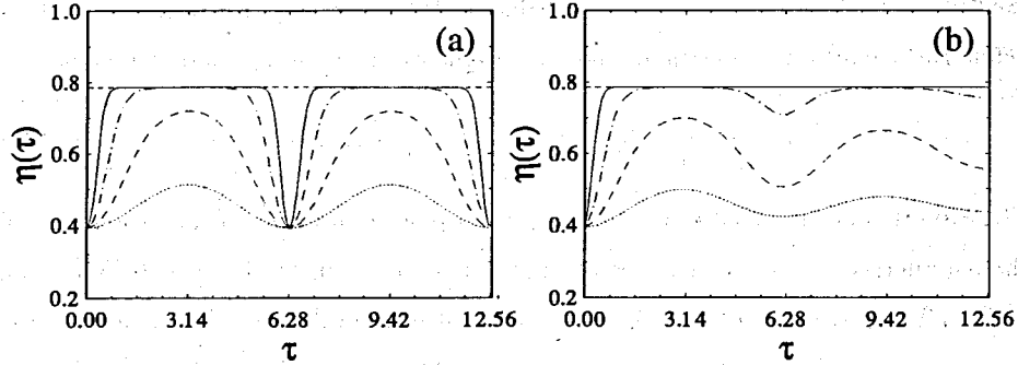
FIG. 2. Evolution of the ellipticity \eta(\tau) , for \eta = \pi/8 .
