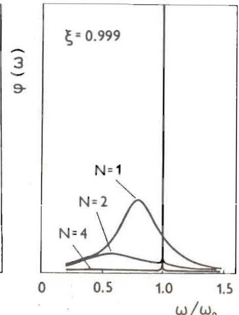
Fig.2. Spectral line \Phi(\omega) for N = 1, 2 and 4 when \xi = 0.999 and \Gamma = \Delta = 0.2 \omega_0 .
