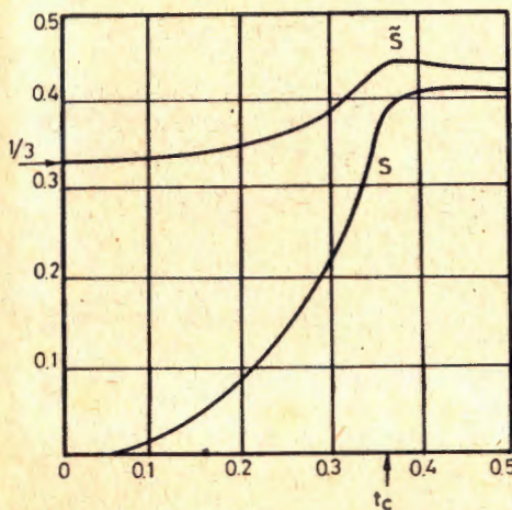
Fig.2. Smoothness s and reduced smoothness \bar{s} against fugacity.
