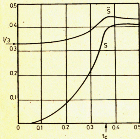
Fig.2. Smoothness s and reduced smoothness \tilde{s} against fugacity.
