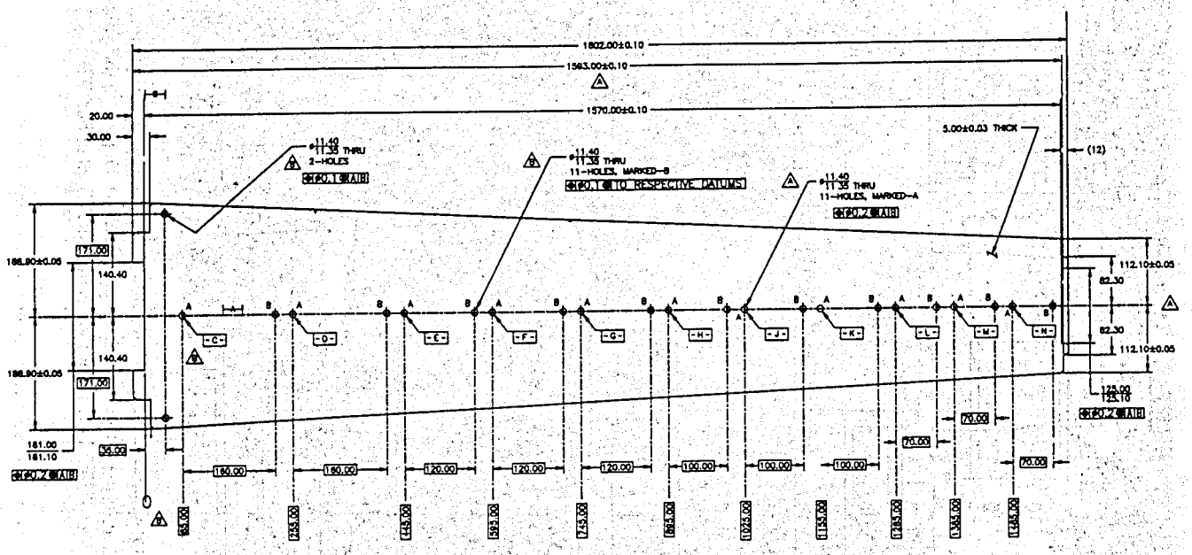
Fig. 2. Master plate.
