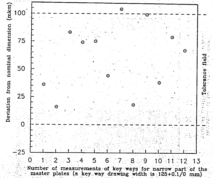
Fig. 11. Key way "measured - nominal" widths distribution for the master plate narrow part.
