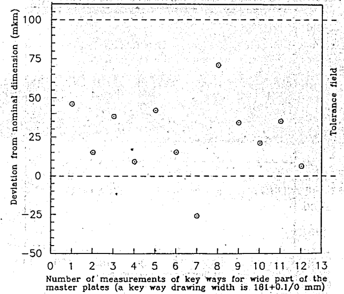
Fig. 12. Key way "measured - nominal" widths distribution for the master plate wide part.
