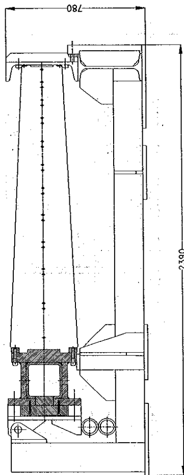
The module0 on the transportation support
