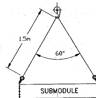
Scheme of submodule slinging with using of lifting eyes
