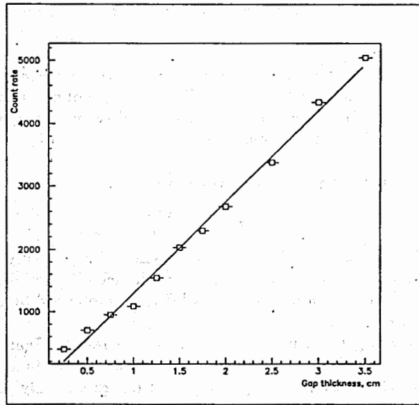
Fig.3 PDT count rate versus collimator width
