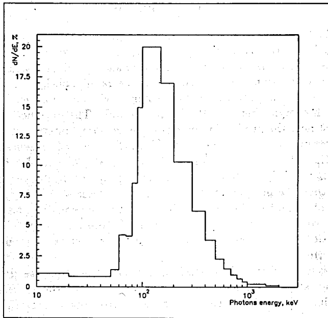
Fig.1 Expected spectrum of background photons
