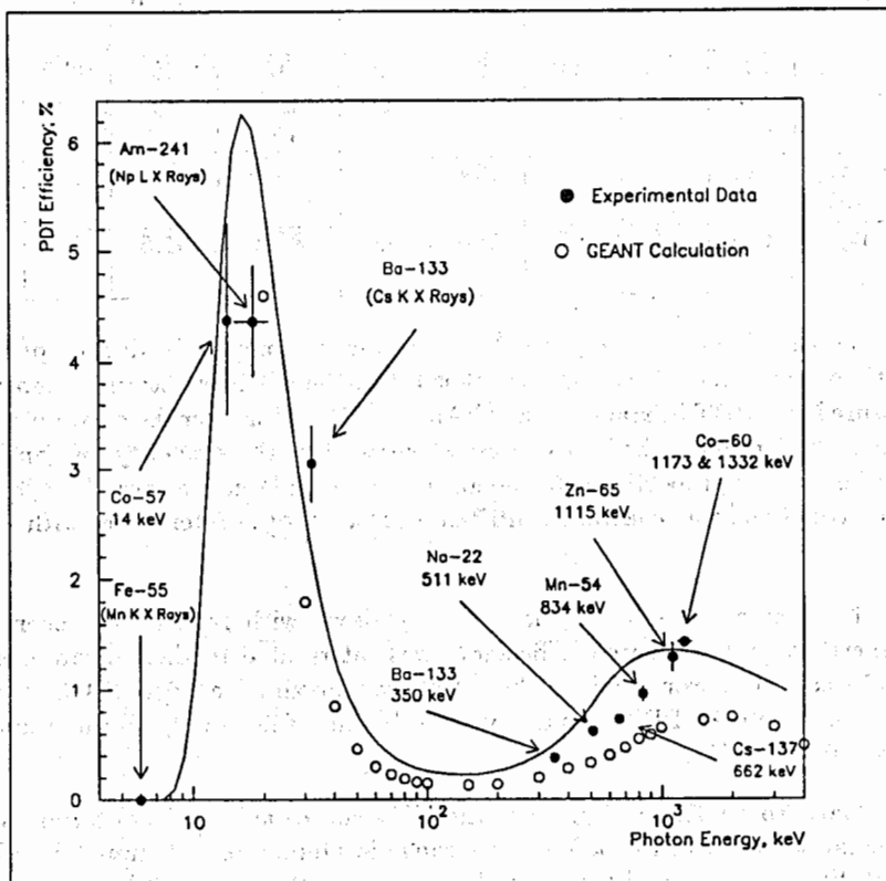
Fig.7 The PDT efficiency versus photon energy
