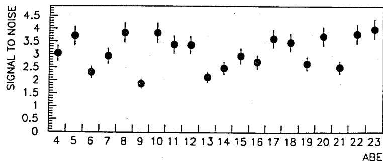
Figure 11: Average ratio of the muon signal and the electronic noise for different absorber elements. The errors shown are the statistical errors only.
