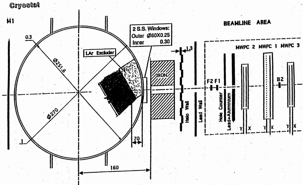
Figure 8: Set-up in the H6 beam line.
