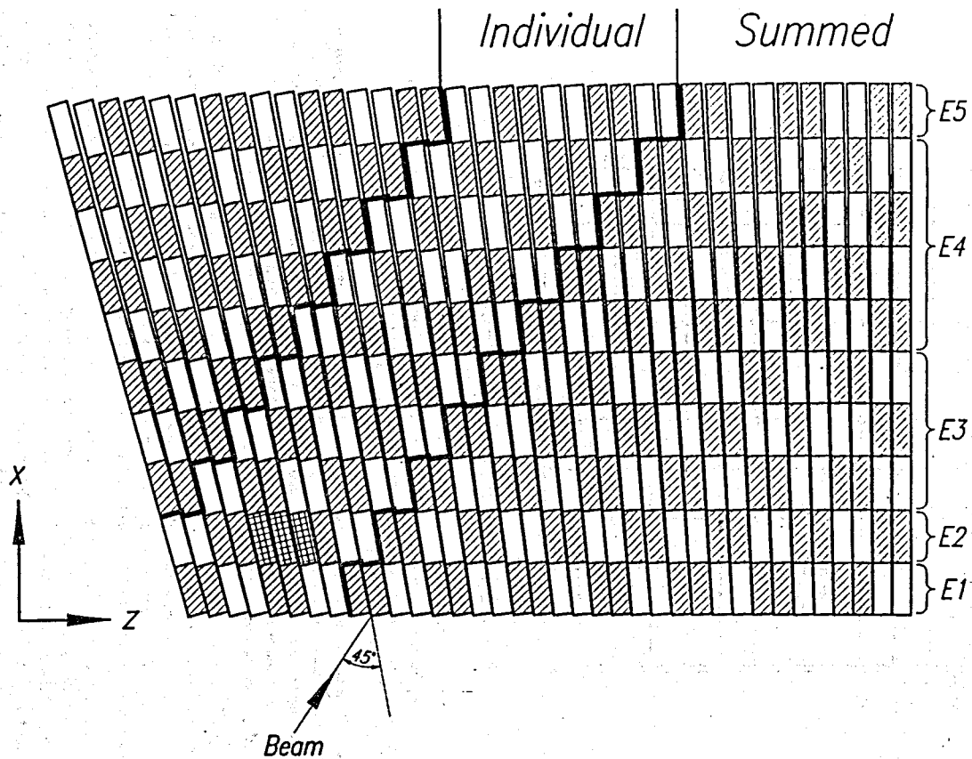
Figure 5: Schematic view of the test module. The cross-hatched pad-groups are equipped with strips. The areas of individual and summed readout are marked. E1 - E5 indicate the longitudinal segmentation.
