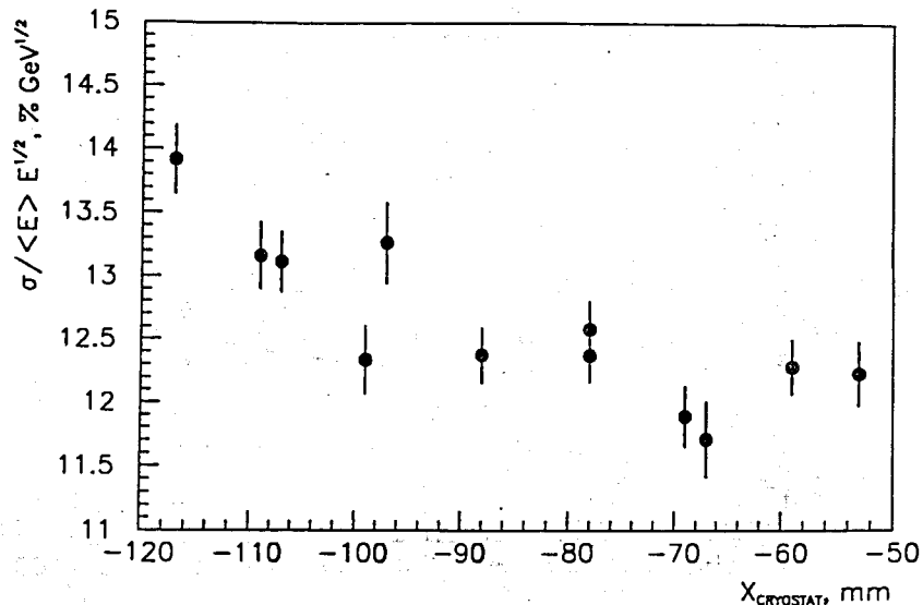
Figure 15: Dependence of the energy resolution [\sigma / \langle E \rangle] \cdot E^{1/2} on the horizontal impact position z for electrons of 40 GeV.
