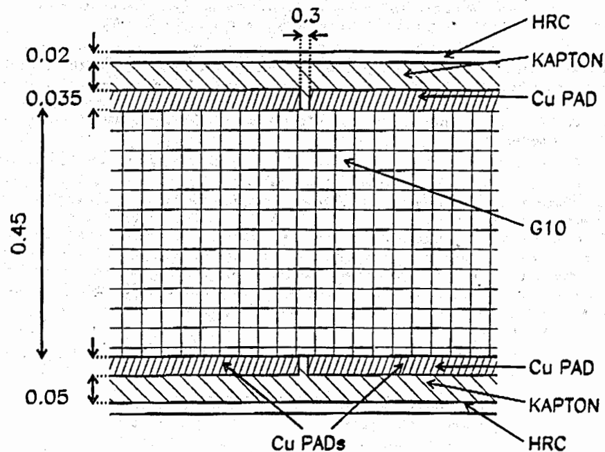
Figure 4: Cross-section of the padboard.
