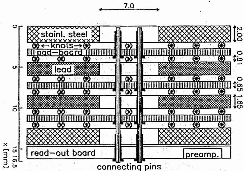
Figure 3: Cross-section of one absorber element showing how the contacts between all padboards and the electronics multilayer board are made.
