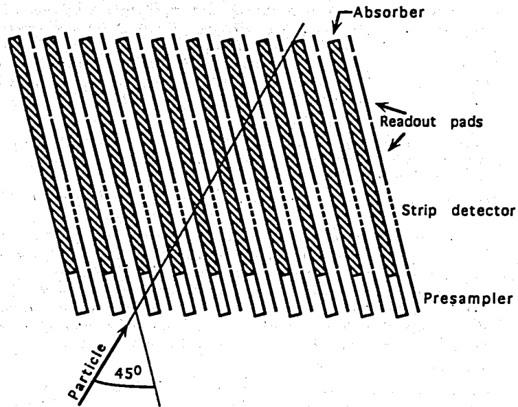
Figure 1: Schematic representation of the TGT concept.
