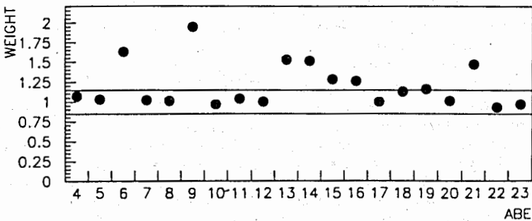
Figure 10: Mean weight for individual absorber elements as given by the average muon response with absorber element 12 as reference.
