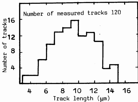
Fig.3. The VH track length spectra.
