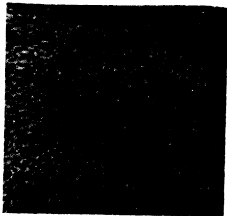
Fig. 1. Microphotograph of VH tracks.
