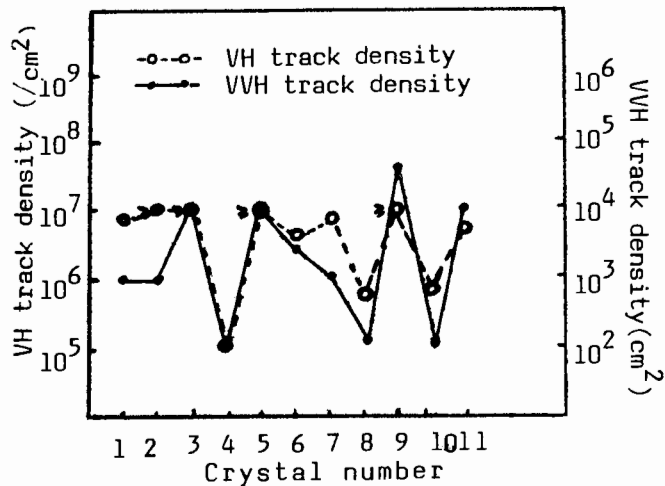
Fig.2. The track density of VH and VVH nuclei in various lunar olivine crystals.
