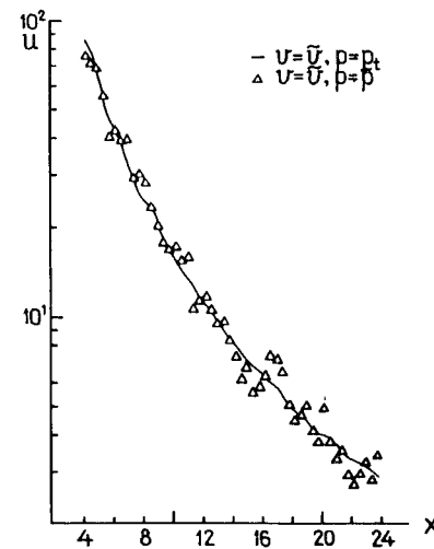
Fig.2. Fluctuations in the iterated solution in the case of +5% error in the RHS and +(5±50)% error in the kernel function.
