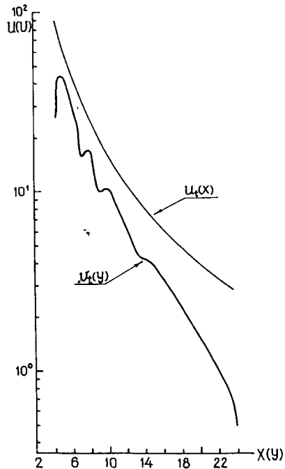
Fig.1. Functions u_t(x) and v_t(y) for the Case 1.
