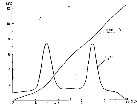
Fig.4. Functions u_t(x) and v_t(y) for the Case 2.
