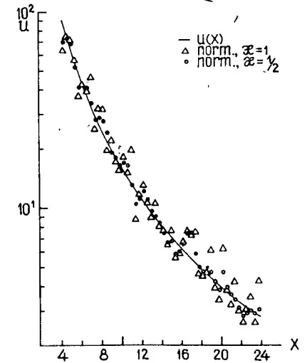
Fig.3. Changes in the stability of the iterated solution applying smoothing transformations to the kernel function.
