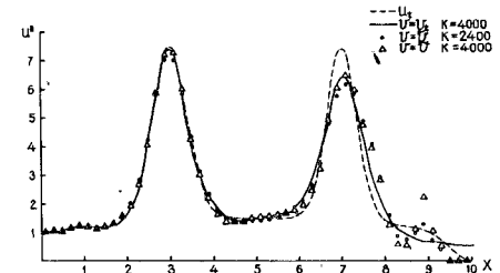
Fig.5. Comparison of fluctuations excited by \pm 5\% of the RHS for large numbers of iterations.
