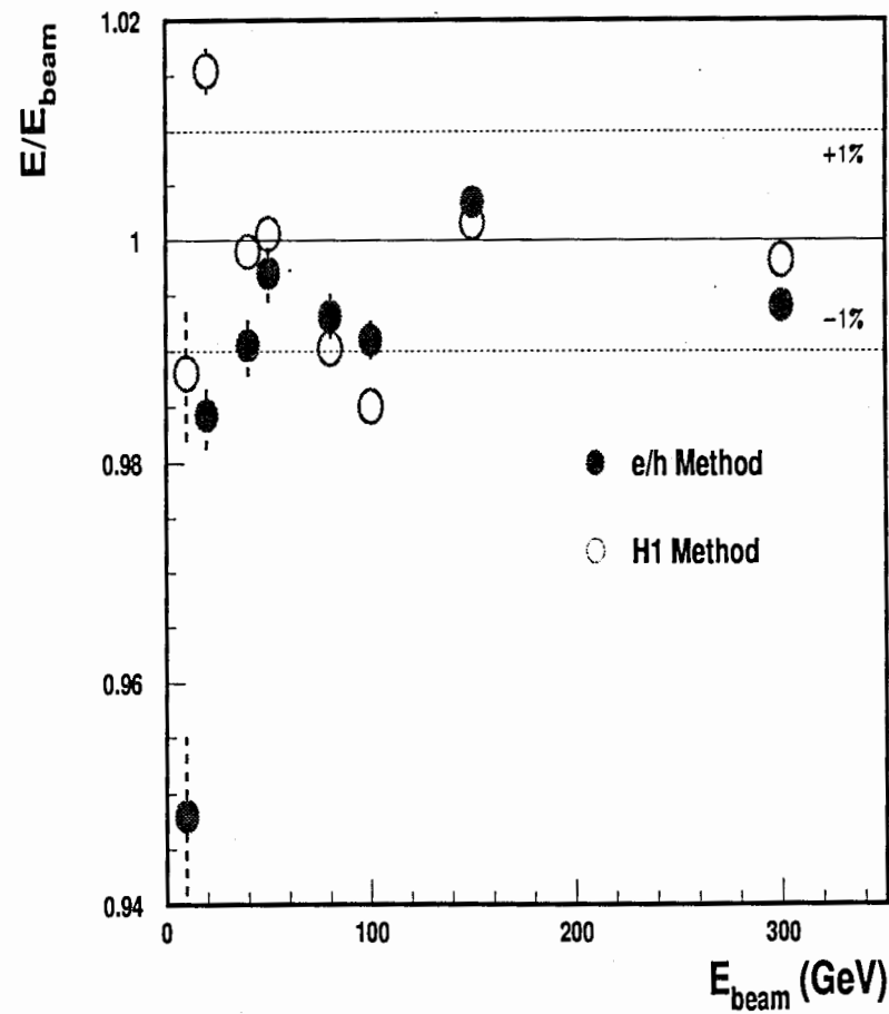
Figure 3: The demonstration of the correctness of the reconstruction of the mean values of energies by the e/h method (black circles): the energy linearity, E_{rec}/E_{beam} as a function of the beam energy. It is also shown the same for the cells weighting H1 method (open circles).
