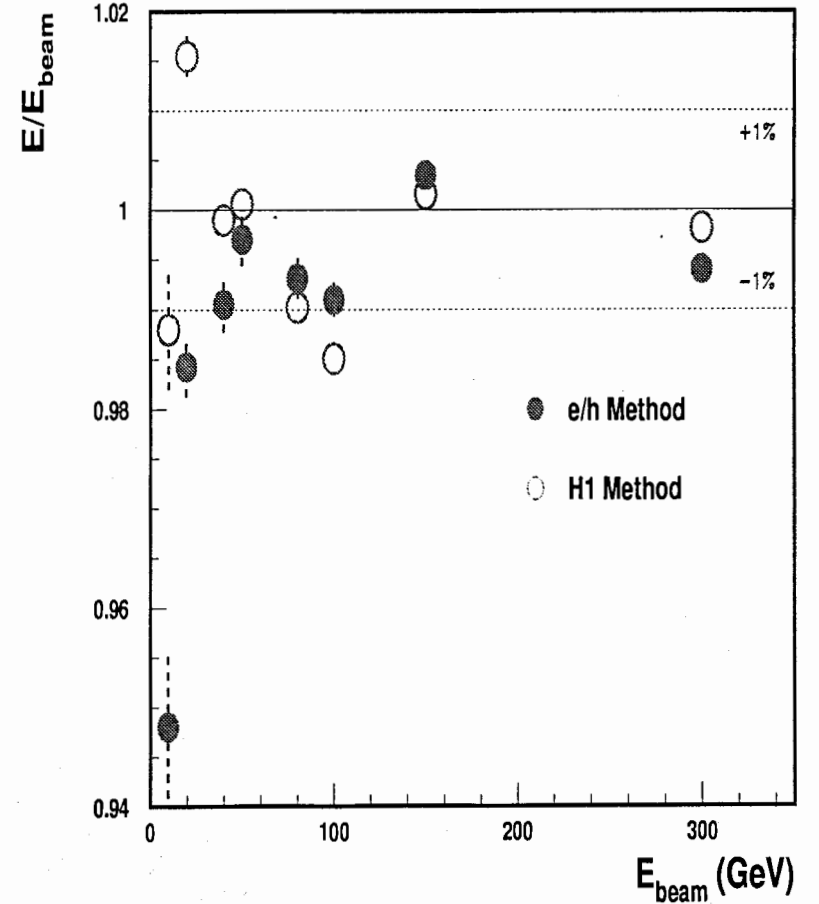
Figure 6: Energy linearity as a function of the beam energy for the e/h method (black circles) and the cells weighting method (open circles).
