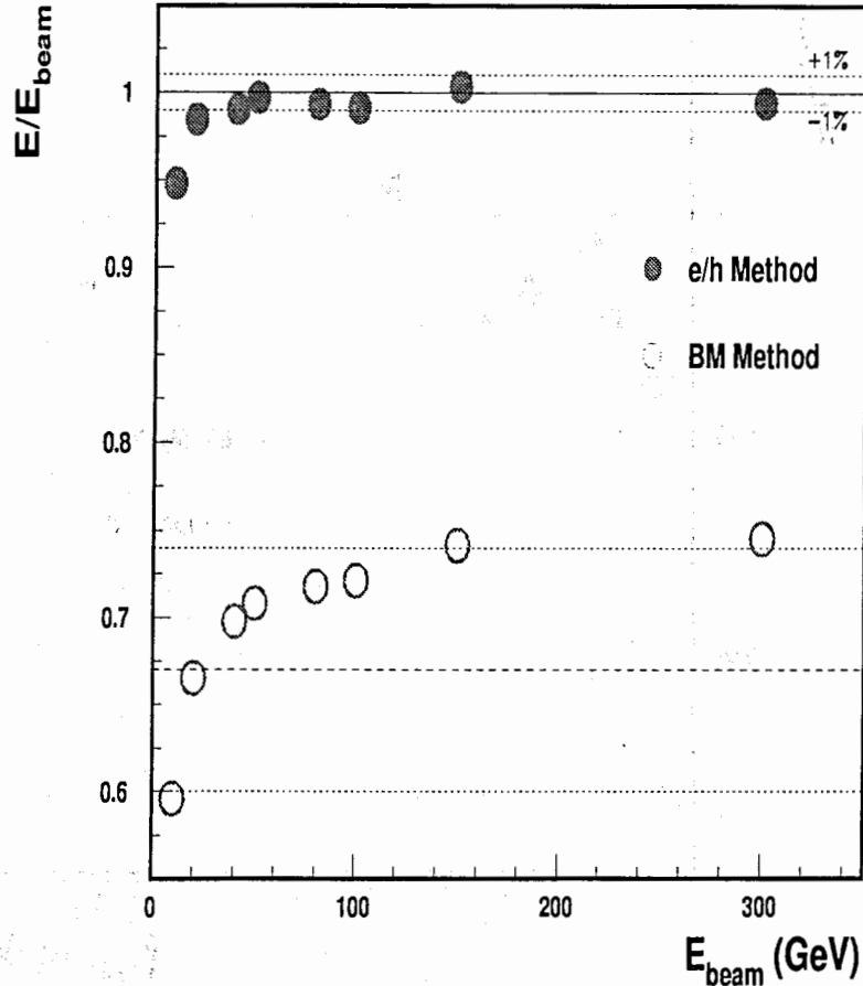
Figure 7: Energy linearity as a function of the beam energy for the e/h method (black circles) and the benchmark method (open circles).
