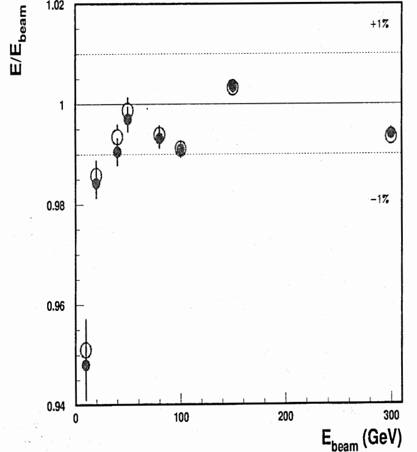
Figure 2: Energy linearity as a function of the beam energy for the e/h method obtained using the iteration procedure with \epsilon = 0.1\% (black circles) and the first approximation (open circles).
