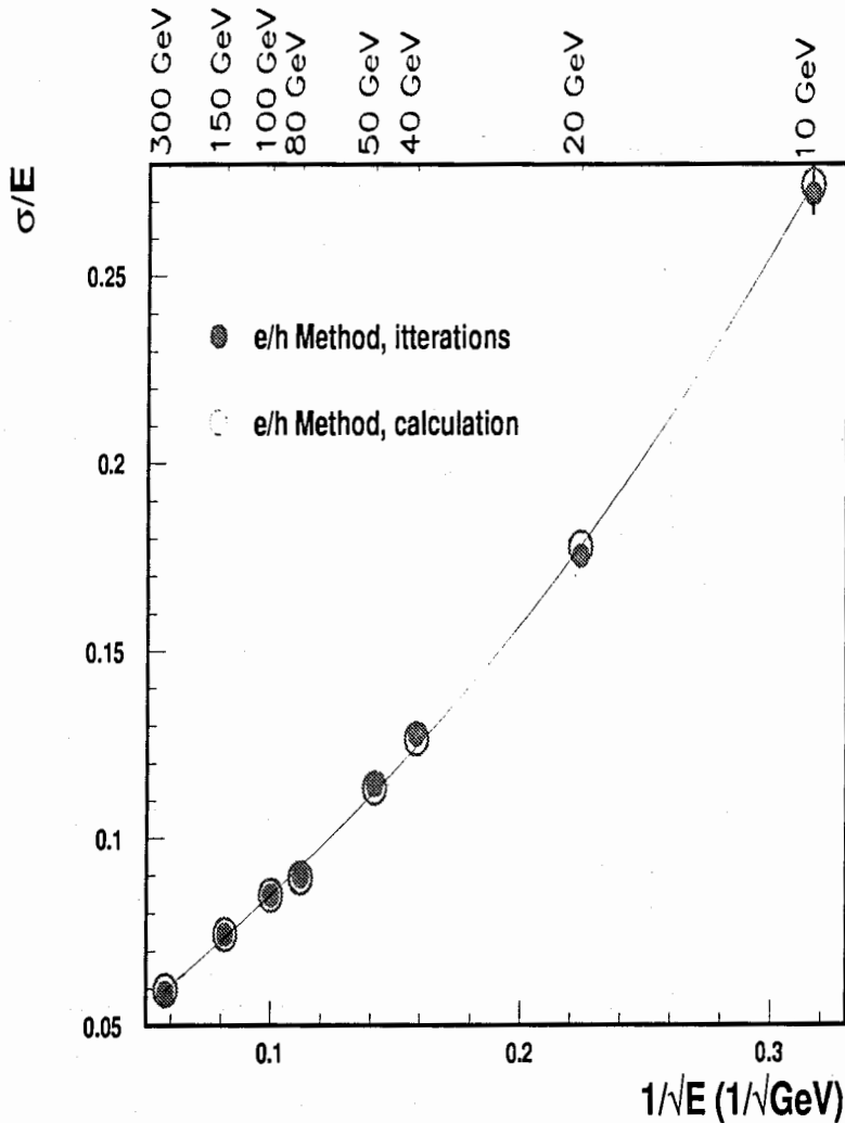
Figure 3: The fractional energy resolutions obtained with the e/h method (black circles), and the first approximation (open circles).
