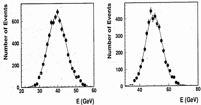
Figure 4: The energy distributions for E_{beam} = 10, 40 GeV (left column, up to down) and E_{beam} = 20, 50 GeV (right column, up to down).
