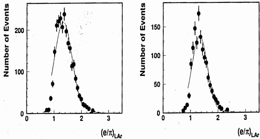
Figure 5: The distributions of the (e/\pi)_{LAR} ratio for E_{beam} = 10, 40 GeV (left column, up to down) and E_{beam} = 20, 50 GeV (right column, up to down).
