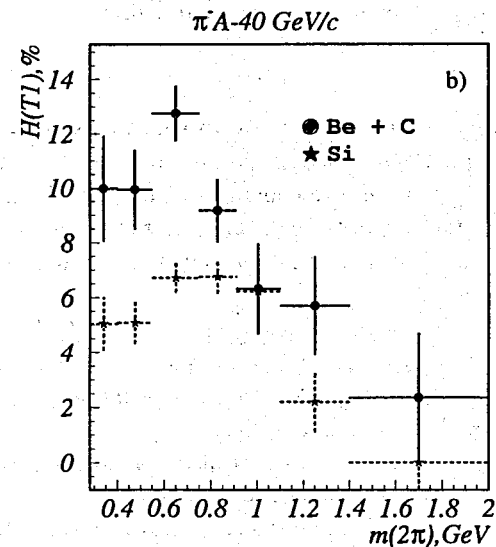
Fig.3. The handedness dependence on m_{3\pi} (a) and m_{\pi^+\pi^-} (b).
