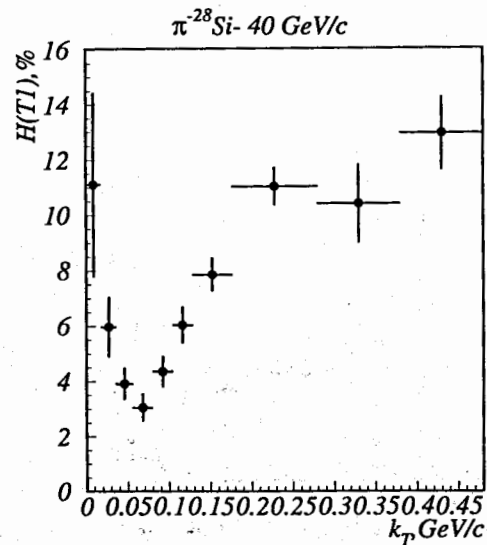
Fig.4. The k_T -dependence of the handedness.
