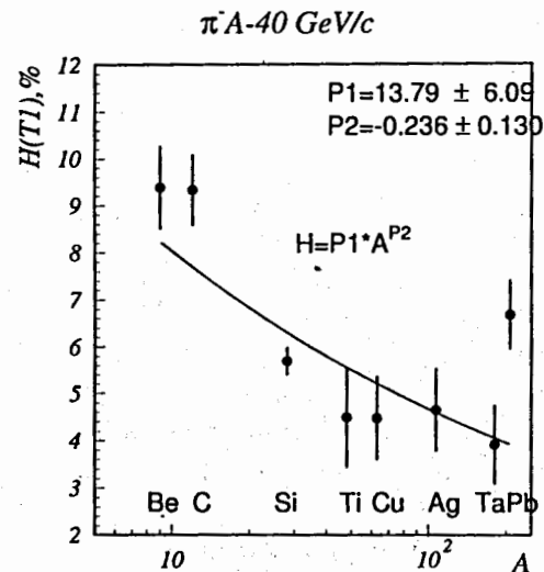
Fig.1. The A -dependence of the handedness.
