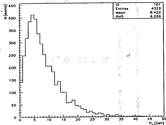
Figure 9: Spectrum of \mu^- from D_s \rightarrow \mu^- \nu decays.
