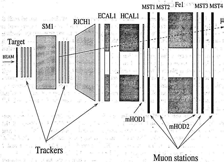
Figure 1: The Large Angle Spectrometer of the COMPASS setup.
