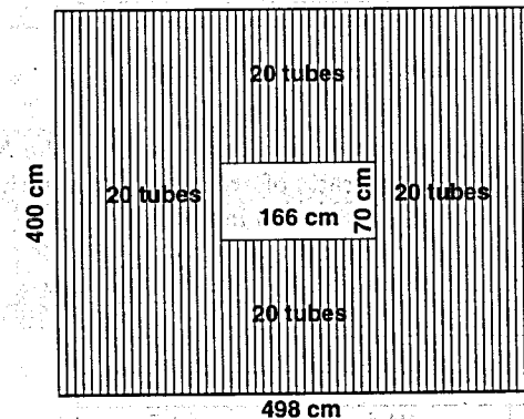
Figure 2: Design of the X and Y planes.
