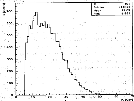
Figure 10: Spectrum of muons from J/\psi \rightarrow \mu^+ \mu^- decays.
